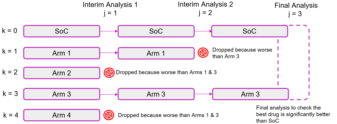
Figure 2: Illustration of the (4:2:1) "Drop-the-Losers" design. Treatments are evaluated at each interim analysis. Treatments with the least promising results are dropped, while the most promising treatments continue to the next stage. The process continues until the final analysis, where the remaining treatment is compared to the control.
