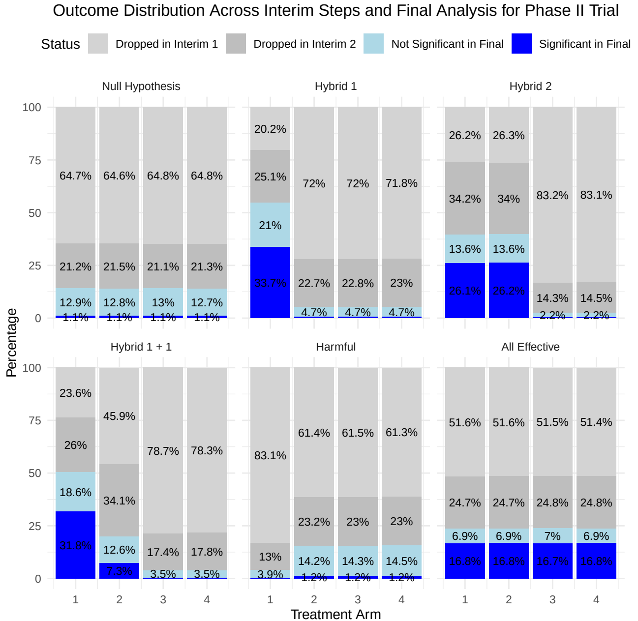
Figure 7: Outcome distribution across interim steps and final analysis for different scenarios for Phase II Trial. In the visualization, percentages below 1% are omitted to improve clarity and avoid overcrowding, as such small values can make the chart difficult to interpret. However, for the Null Hypothesis, all percentages are displayed regardless of their size to ensure full visibility. Additionally, all results, including those below 1%, are fully available in Table 7 for detailed examination.
