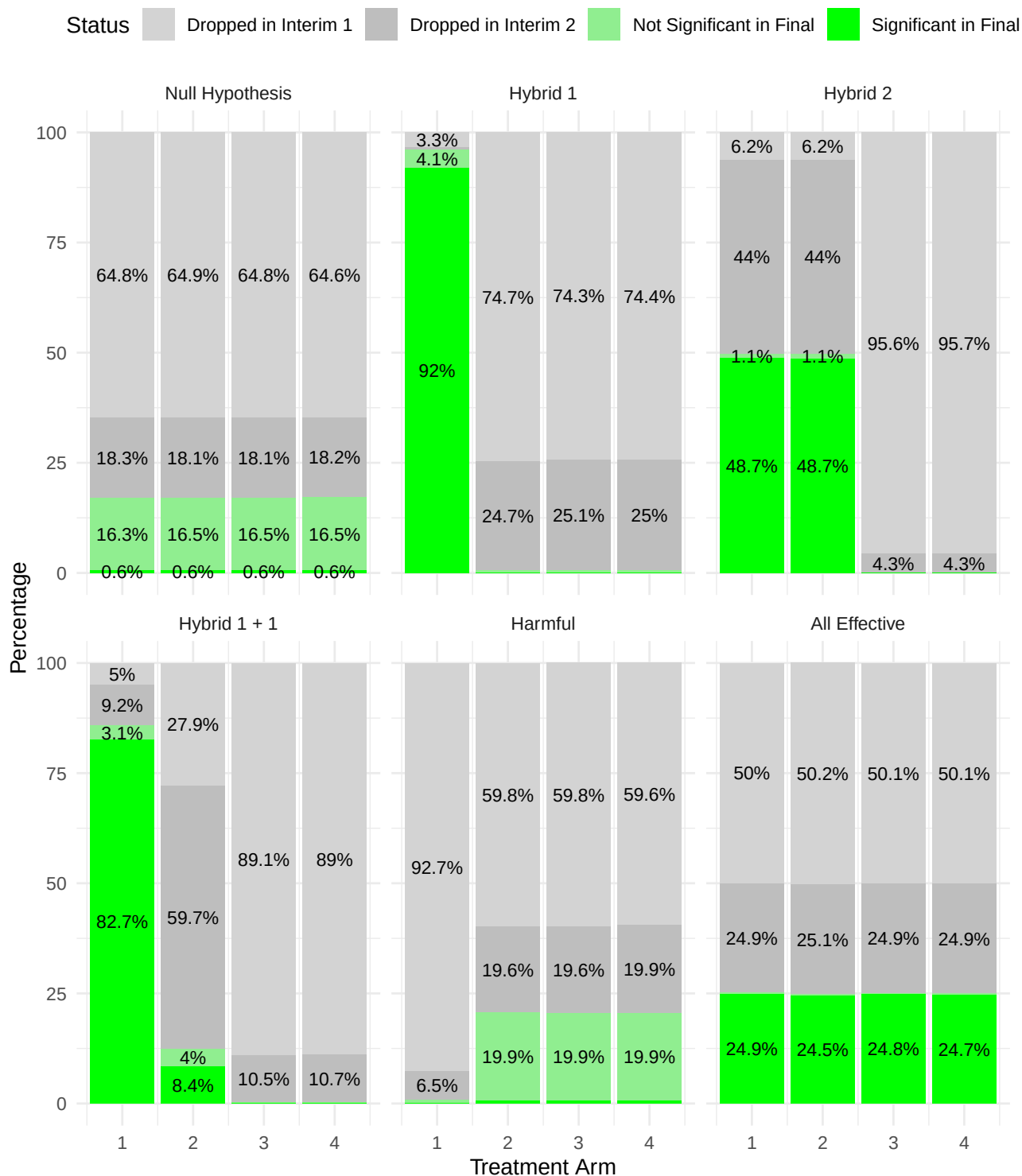
Figure 6: Outcome distribution across interim steps and final analysis for different scenarios for Phase III Trial. In the visualization, percentages below 1% are omitted to improve clarity and avoid overcrowding, as such small values can make the chart difficult to interpret. However, for the Null Hypothesis, all percentages are displayed regardless of their size to ensure full visibility. Additionally, all results, including those below 1%, are fully available in Table 6 for detailed examination.
