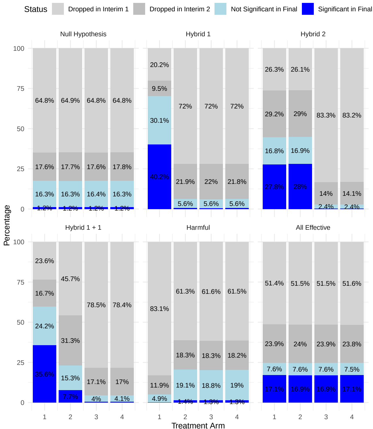
Figure 5: Outcome distribution across interim steps and final analysis for different scenarios for Phase II Trial. In the visualization, percentages below 1% are omitted to improve clarity and avoid overcrowding, as such small values can make the chart difficult to interpret. However, for the Null Hypothesis, all percentages are displayed regardless of their size to ensure full visibility. Additionally, all results, including those below 1%, are fully available in Table 3 for detailed examination.
