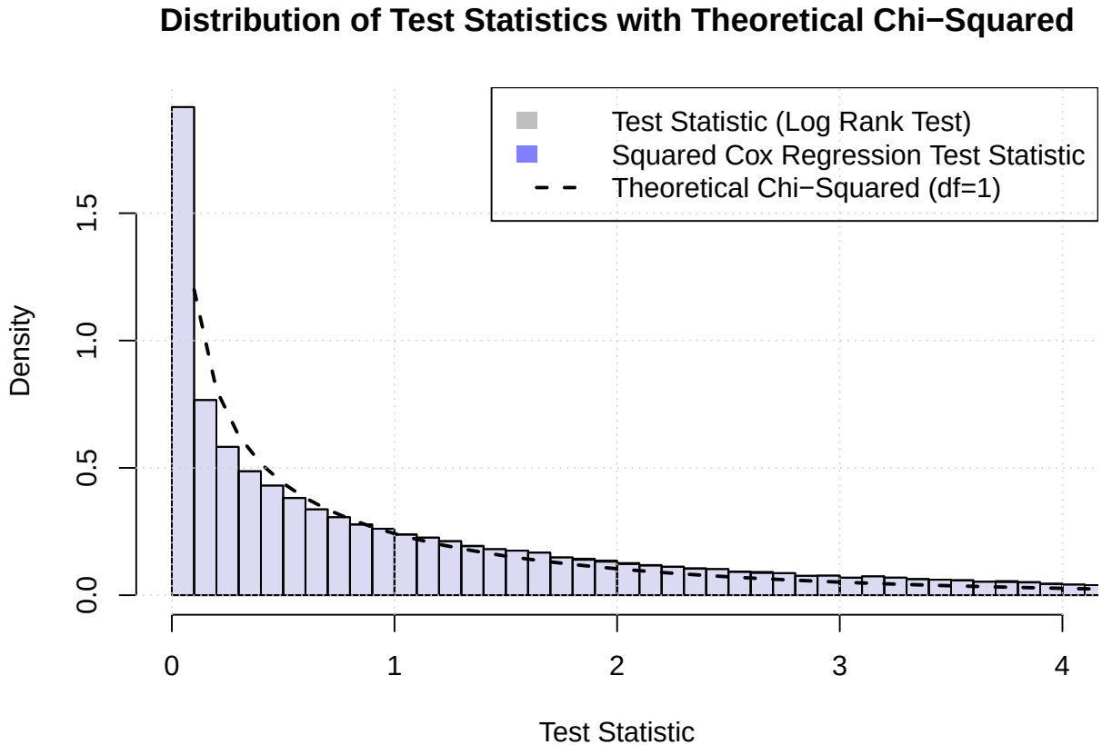
Figure 4: Distribution of Test Statistics with Theoretical Chi-Squared ( \chi^2_{(1)} ). The gray bars represent Log-Rank test statistics, the blue bars represent squared Cox regression test statistics, and the dashed line represents the theoretical \chi^2_{(1)} distribution.
