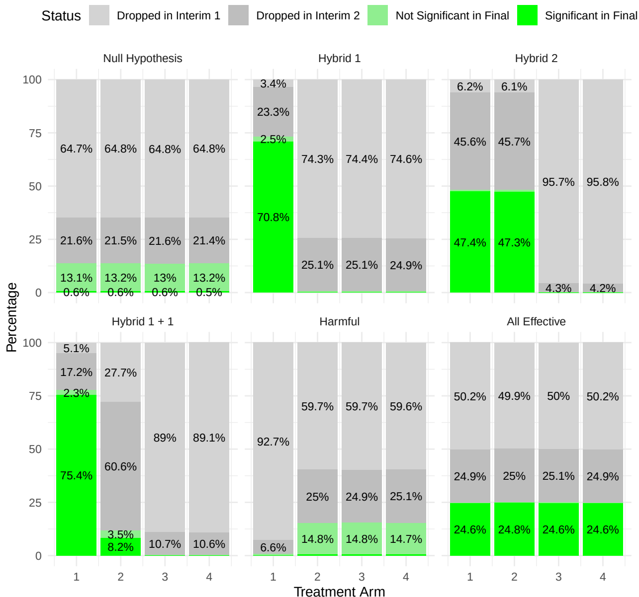
Figure 8: Outcome distribution across interim steps and final analysis for different scenarios for Phase III Trial. In the visualization, percentages below 1% are omitted to improve clarity and avoid overcrowding, as such small values can make the chart difficult to interpret. However, for the Null Hypothesis, all percentages are displayed regardless of their size to ensure full visibility. Additionally, all results, including those below 1%, are fully available in Table 8 for detailed examination.
