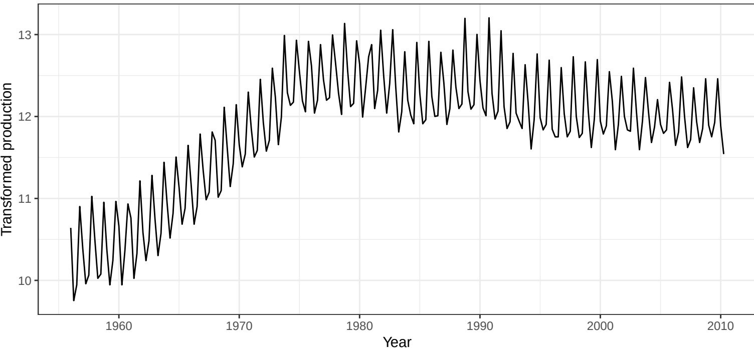
Box-Cox transformed beer (lambda = 0.20)
