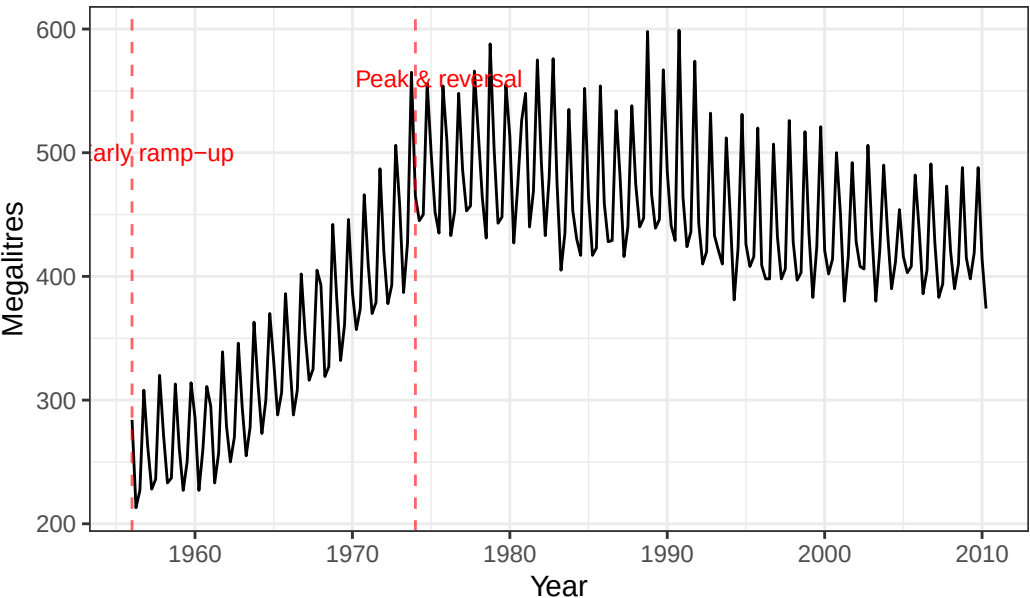
Australian beer production – unusual periods highlighted
