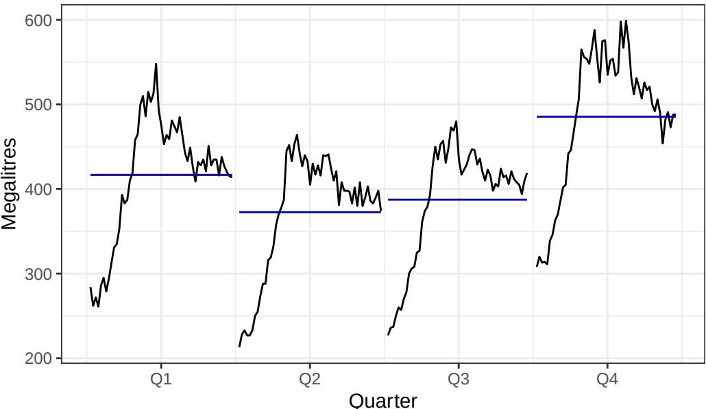
Seasonal subseries – Australian beer production
