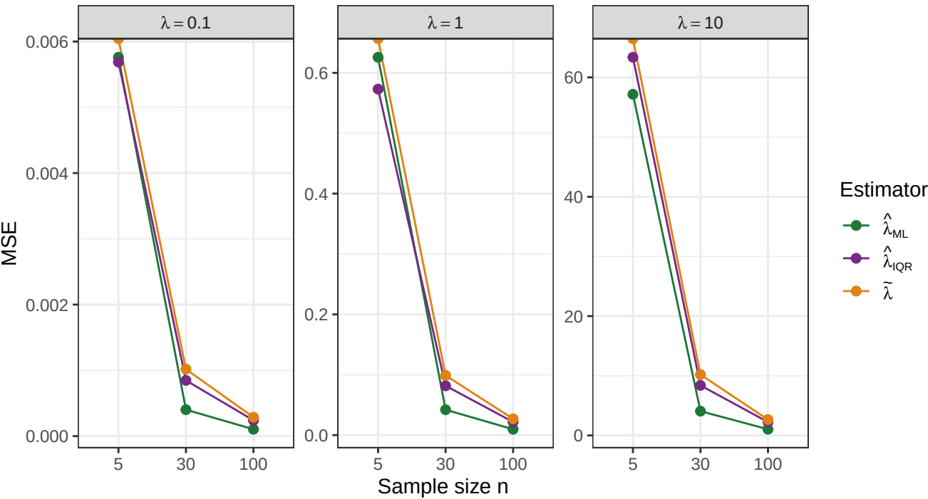
Monte Carlo MSE by estimator, sample size and rate parameter
