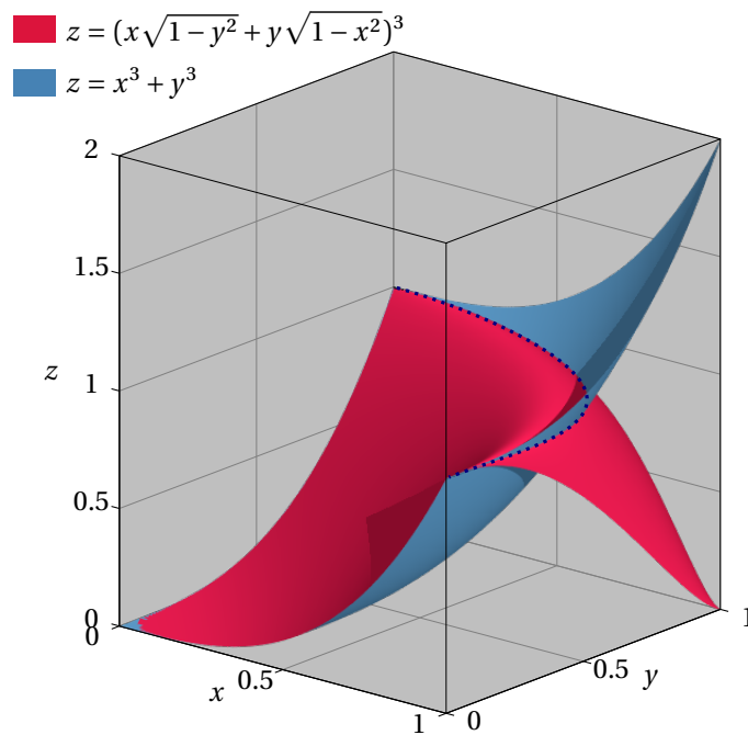
Figure 17: Intersection of two implicit surfaces
