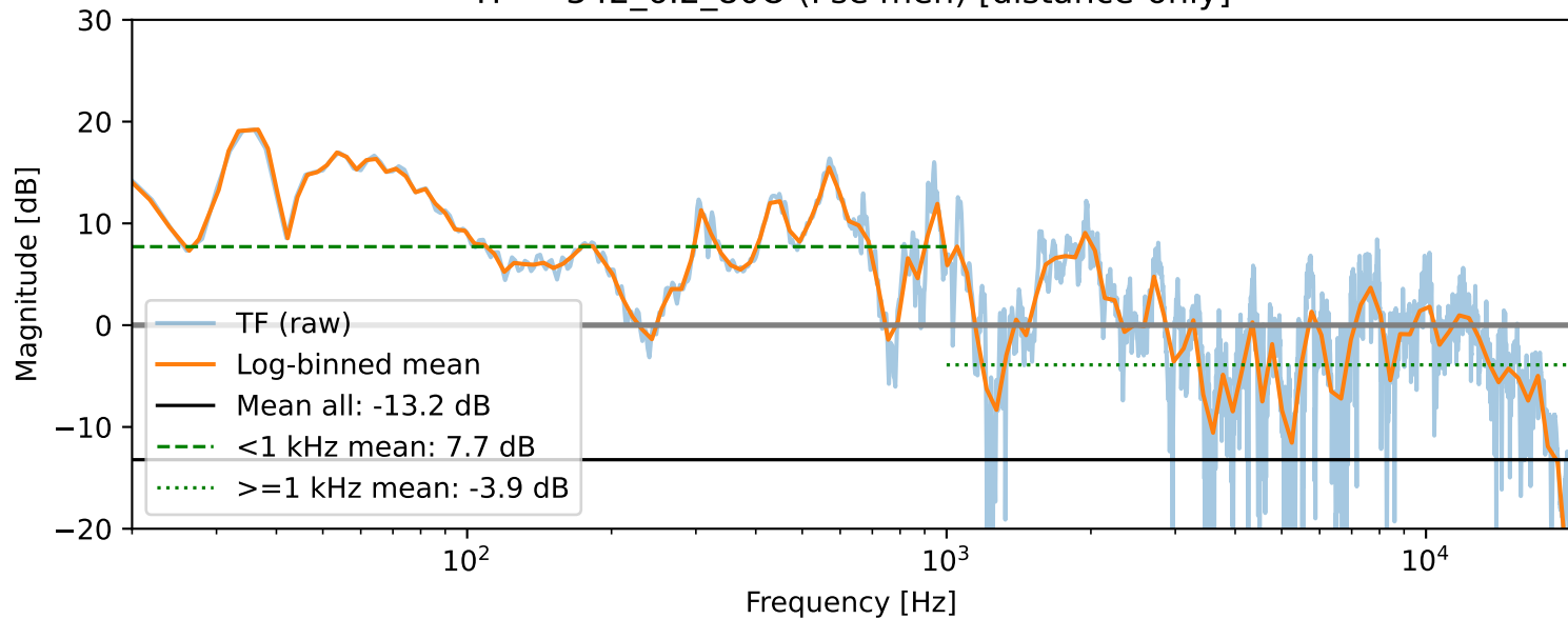
TF — 342_6.2_800 (Pse men) [distance-only]
