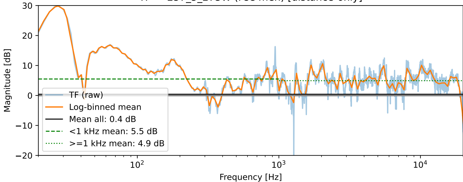
TF — 257_5_273W (Pse men) [distance-only]
