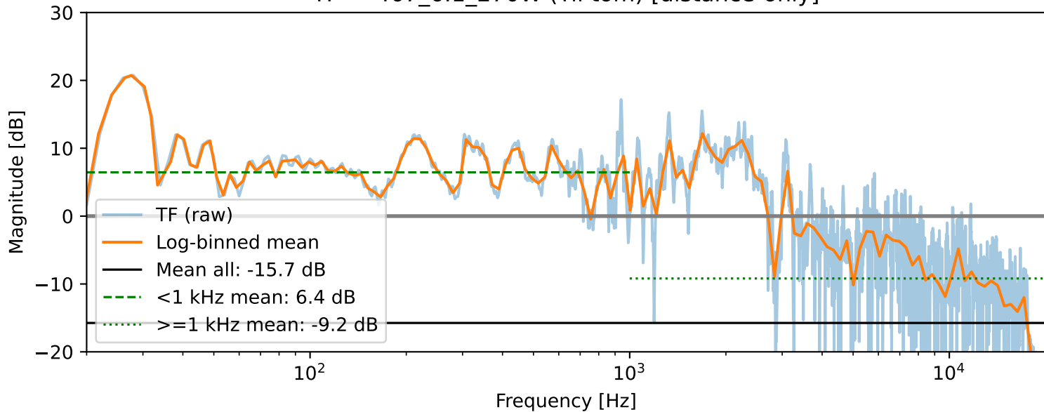
TF — 467_6.1_270W (Til tom) [distance-only]
