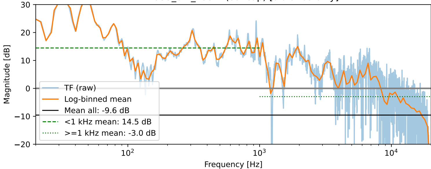
TF — 353_8.1_255W (Sal cap) [distance-only]
