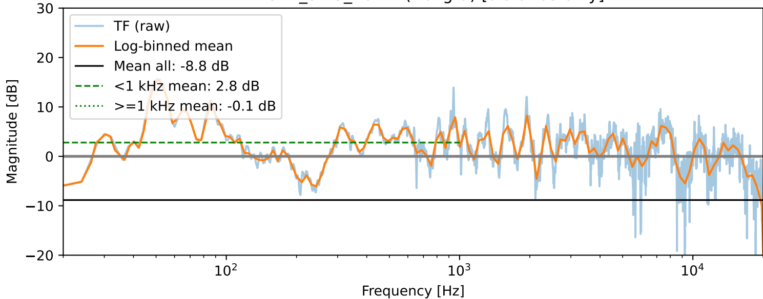
TF — 344_3.15_261W (Abi gra) [distance-only]
