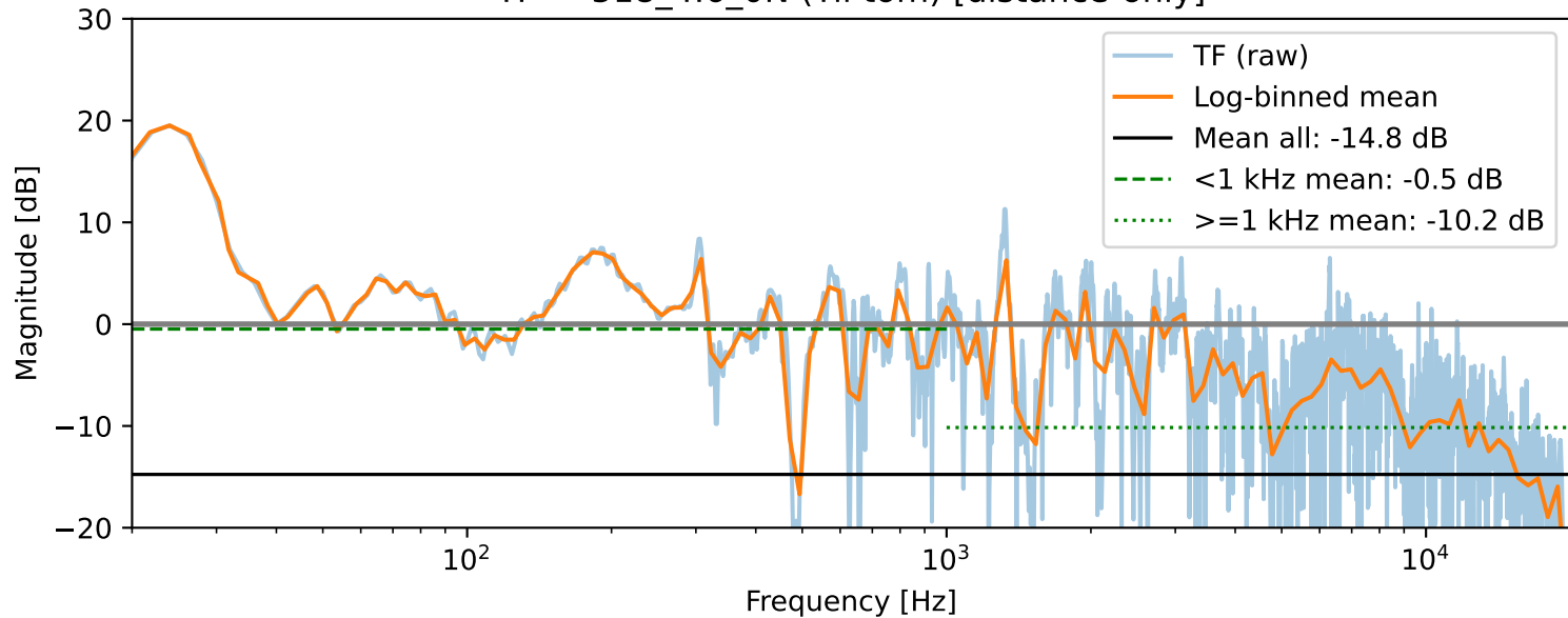
TF — 518_4.6_0N (Til tom) [distance-only]
