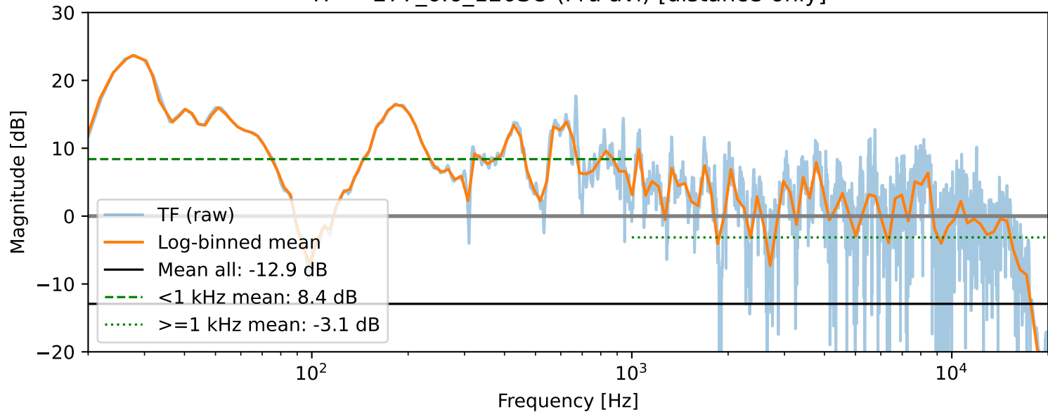
TF — 277_6.6_120SO (Pru avi) [distance-only]
