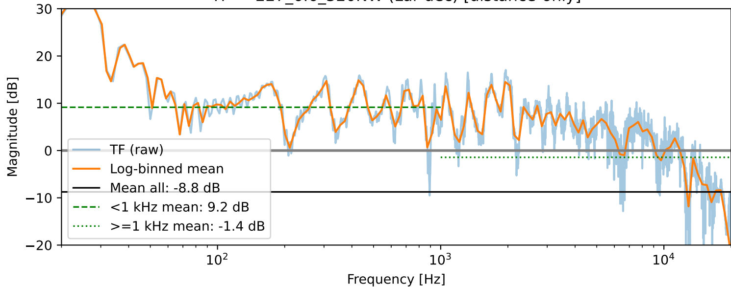
TF — 227_6.6_320NW (Lar dec) [distance-only]
