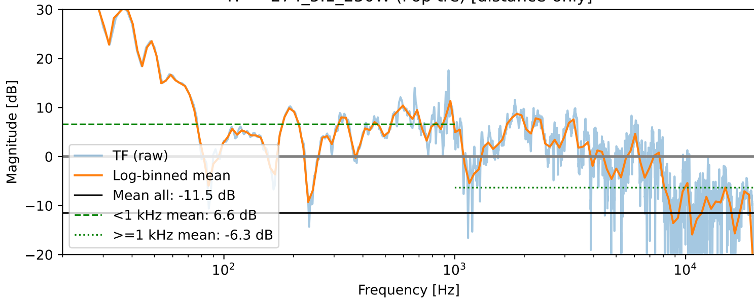
TF — 274_5.1_250W (Pop tre) [distance-only]
