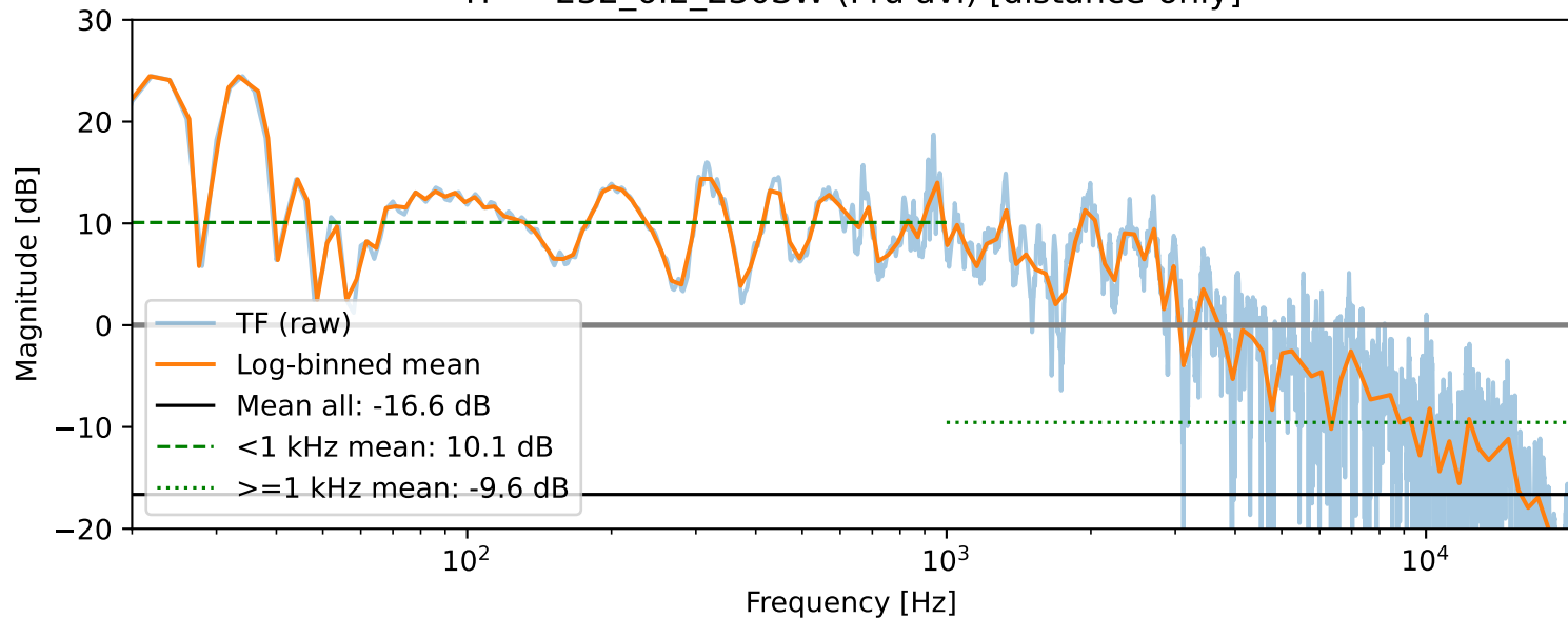
TF — 232_6.2_230SW (Pru avi) [distance-only]
