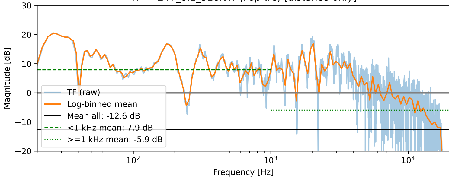
TF — 247_8.2_318NW (Pop tre) [distance-only]
