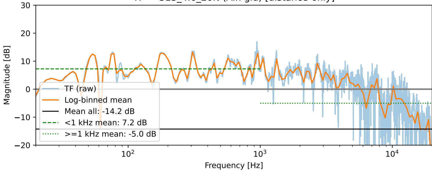
TF — 313_4.6_20N (Aln glu) [distance-only]
