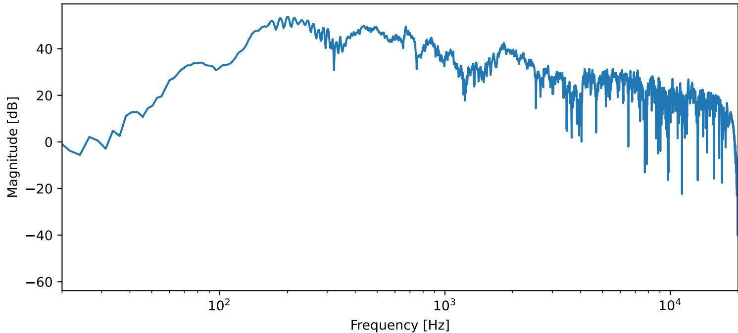
FFT of trimmed recording — 270_5.4_240SW (Aln glu)
