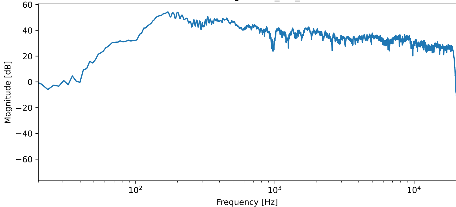
FFT of trimmed recording — 502_3.8_46NO (Ced deo)
