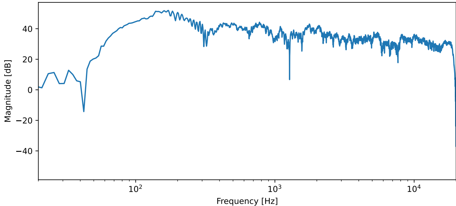
FFT of trimmed recording — 257_5_273W (Pse men)
