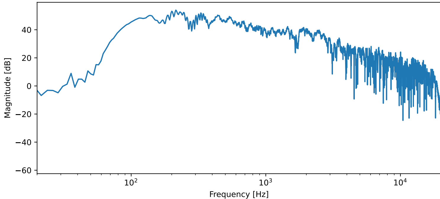
FFT of trimmed recording — 232_6.2_230SW (Pru avi)
