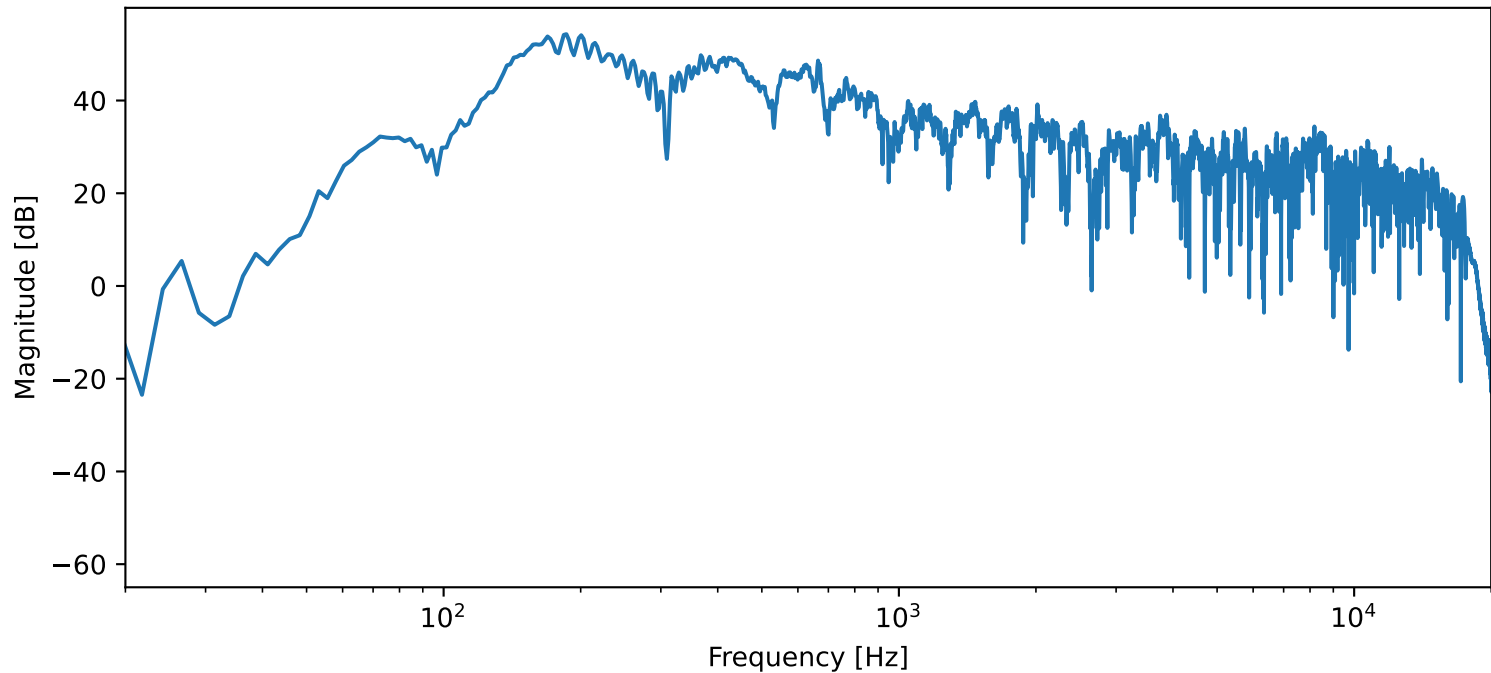
FFT of trimmed recording — 277_6.6_120SO (Pru avi)
