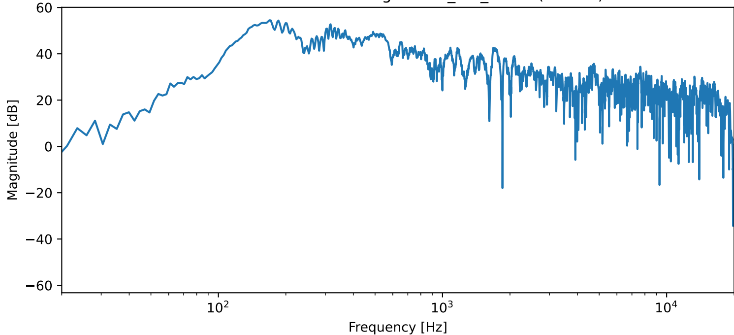
FFT of trimmed recording — 499_4.6_40NO (Til tom)
