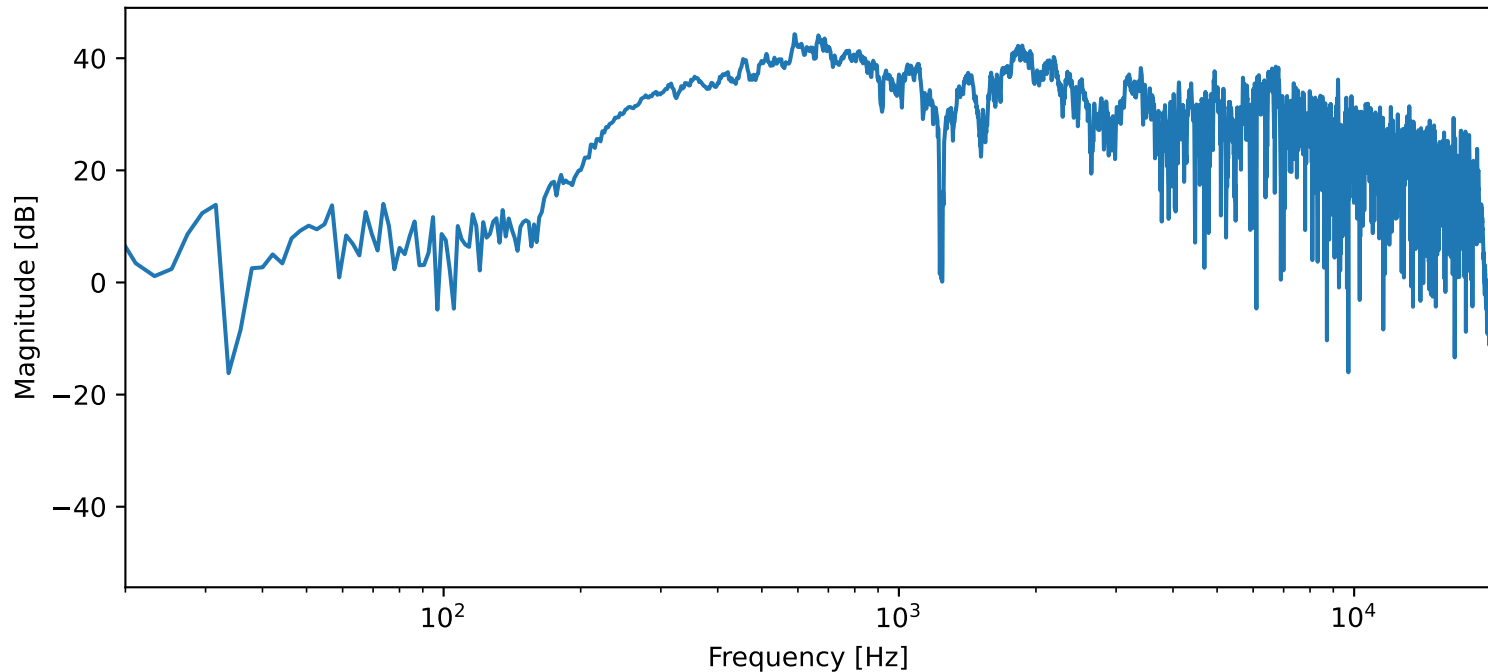
FFT of trimmed recording — 353_8.1_255W (Sal cap)
