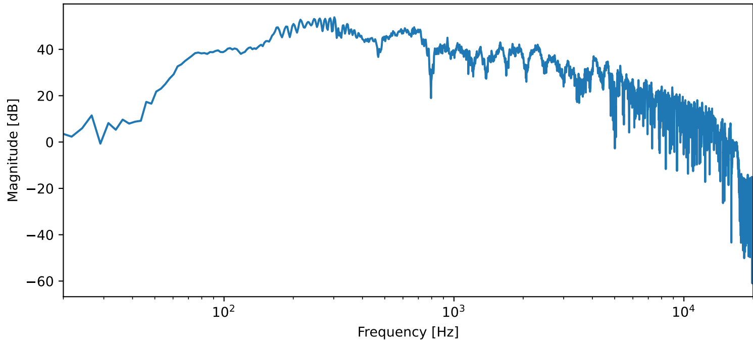
FFT of trimmed recording — 327_9_170S (Sal cap)
