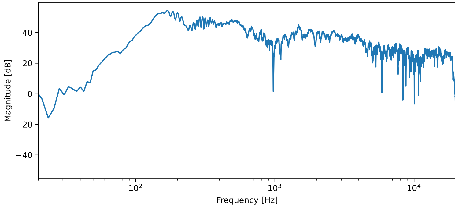
FFT of trimmed recording — 298_4.5_336NW (Abi gra)
