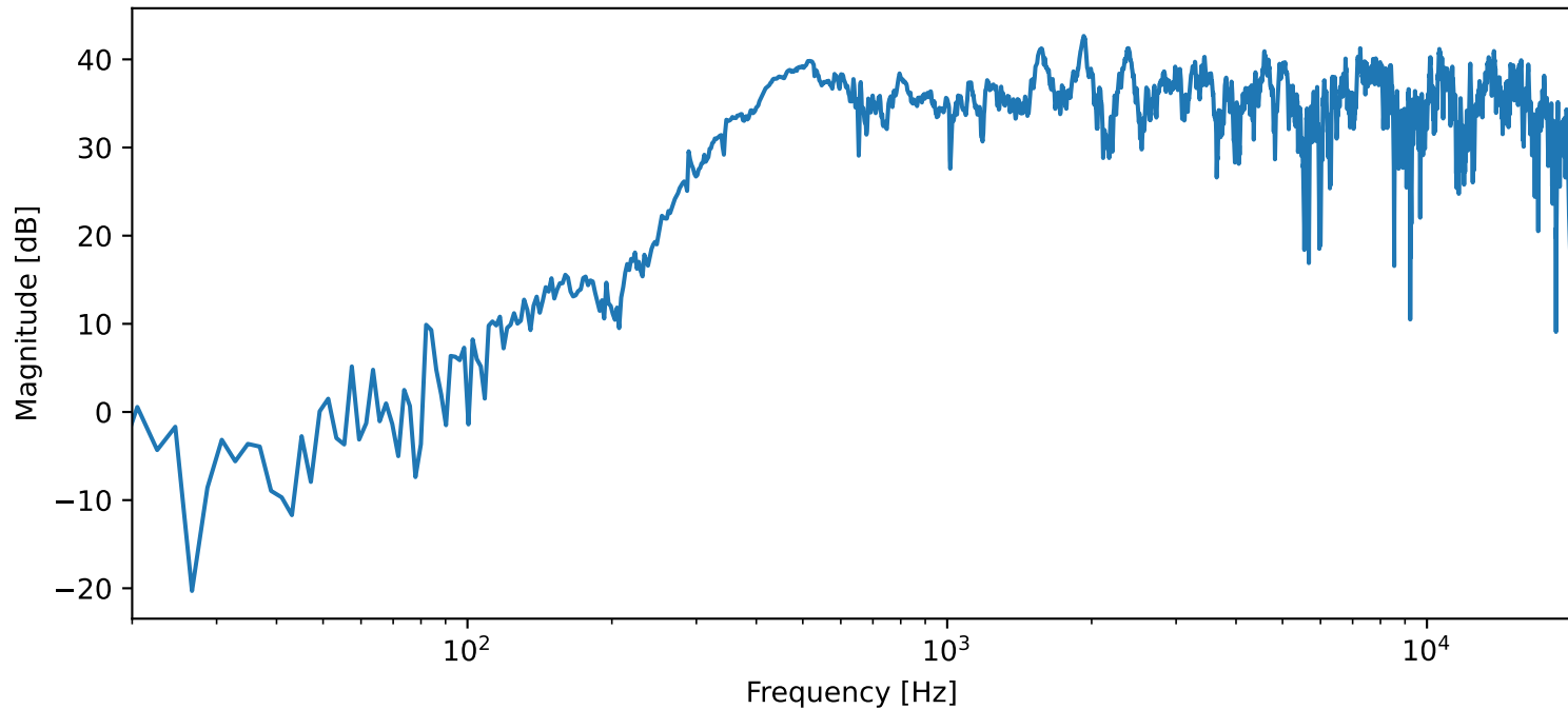
FFT of trimmed recording — 344_3.15_261W (Abi gra)
