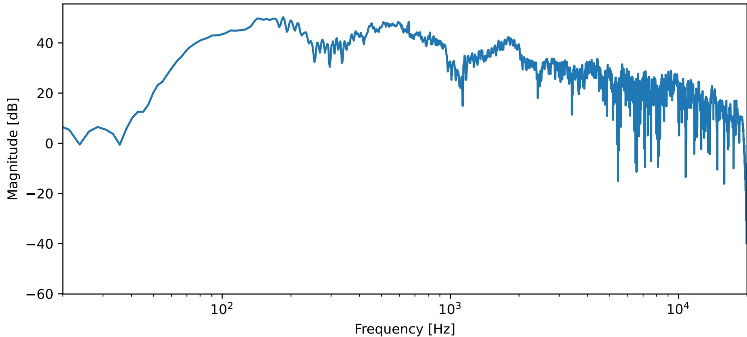
FFT of trimmed recording — 281_5.8_190S (Lar dec)
