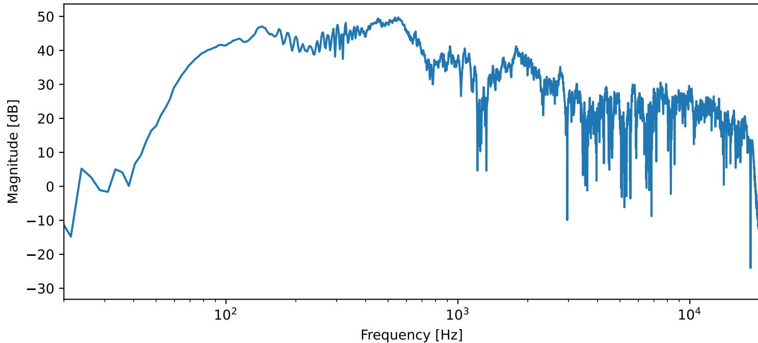
FFT of trimmed recording — 342_6.2_800 (Pse men)
