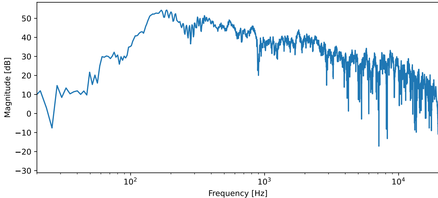
FFT of trimmed recording — 332_5_55NO (Pin nig)
