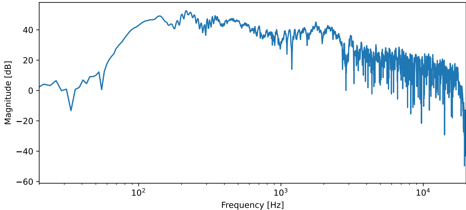
FFT of trimmed recording — 467_6.1_270W (Til tom)
