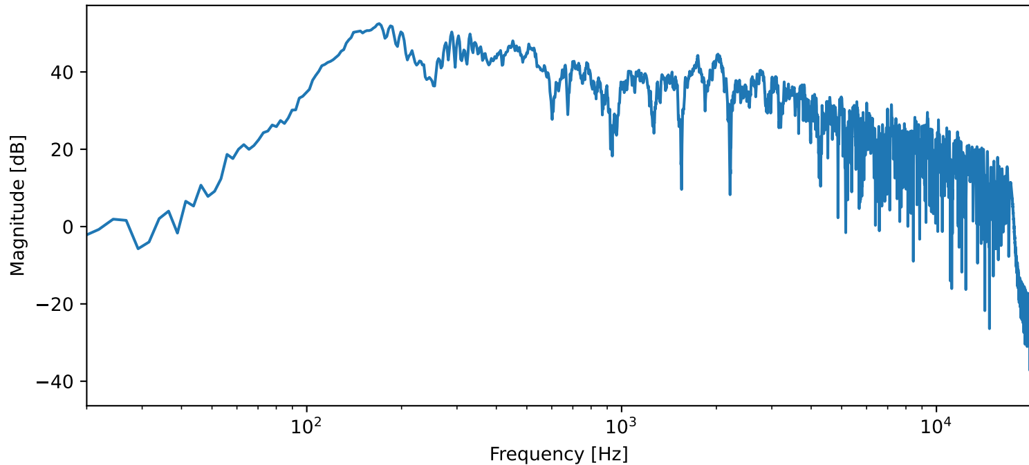
FFT of trimmed recording — 247_8.2_318NW (Pop tre)
