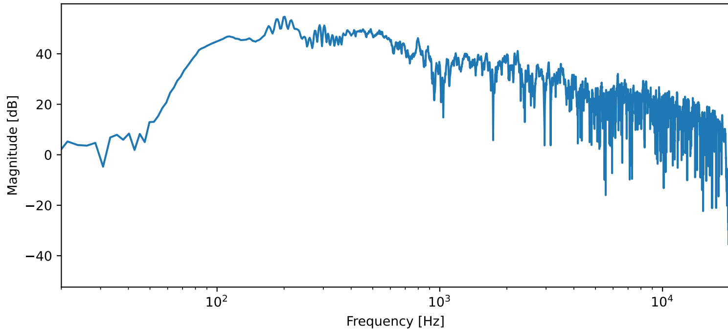
FFT of trimmed recording — 518_4.6_0N (Til tom)
