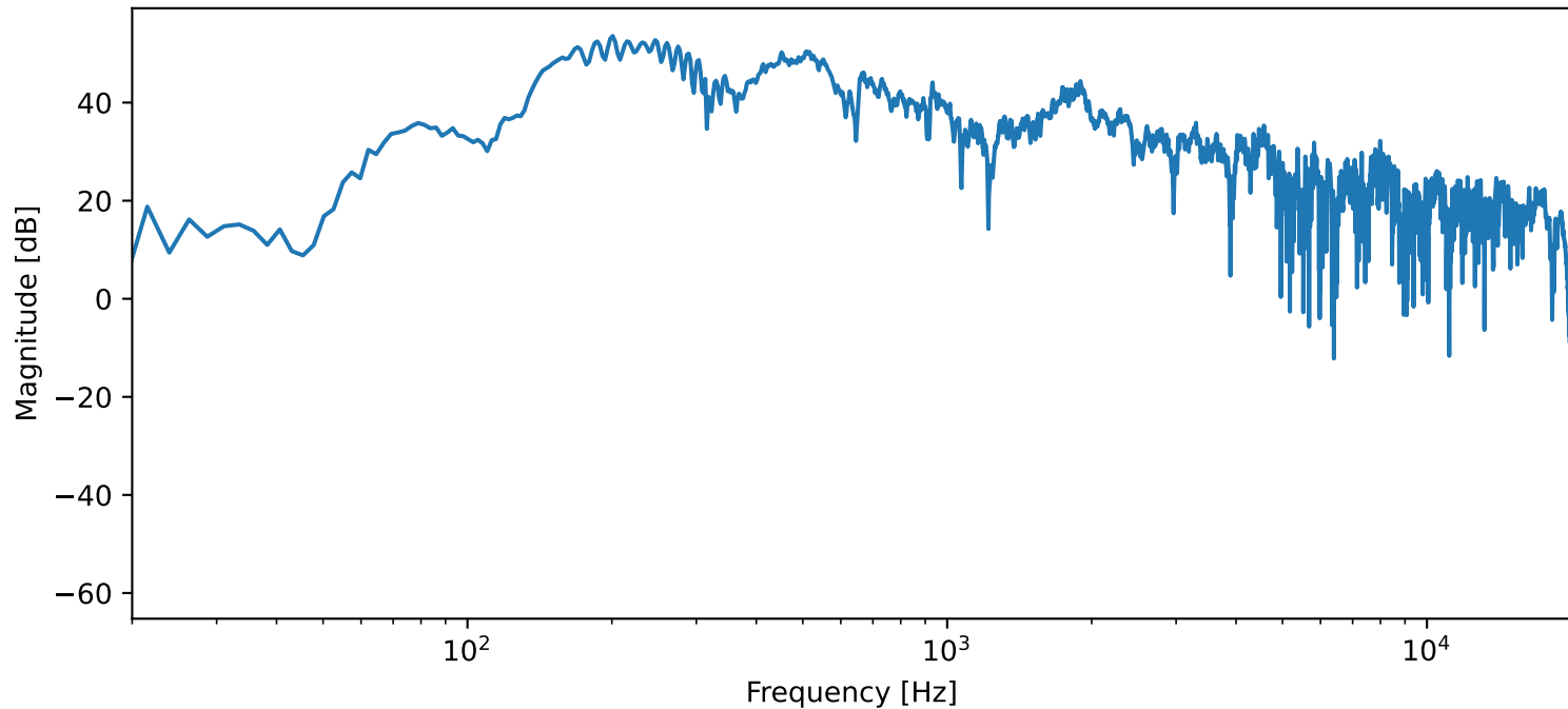
FFT of trimmed recording — 333_6_325NW (Pin nig)
