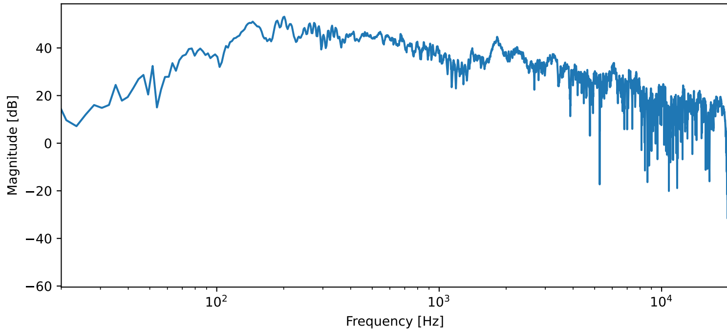
FFT of trimmed recording — 274_5.1_250W (Pop tre)
