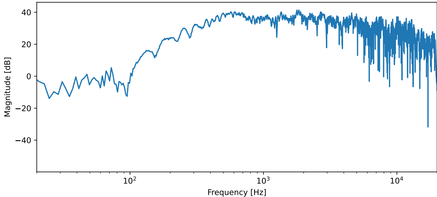
FFT of trimmed recording — 313_4.6_20N (Aln glu)
