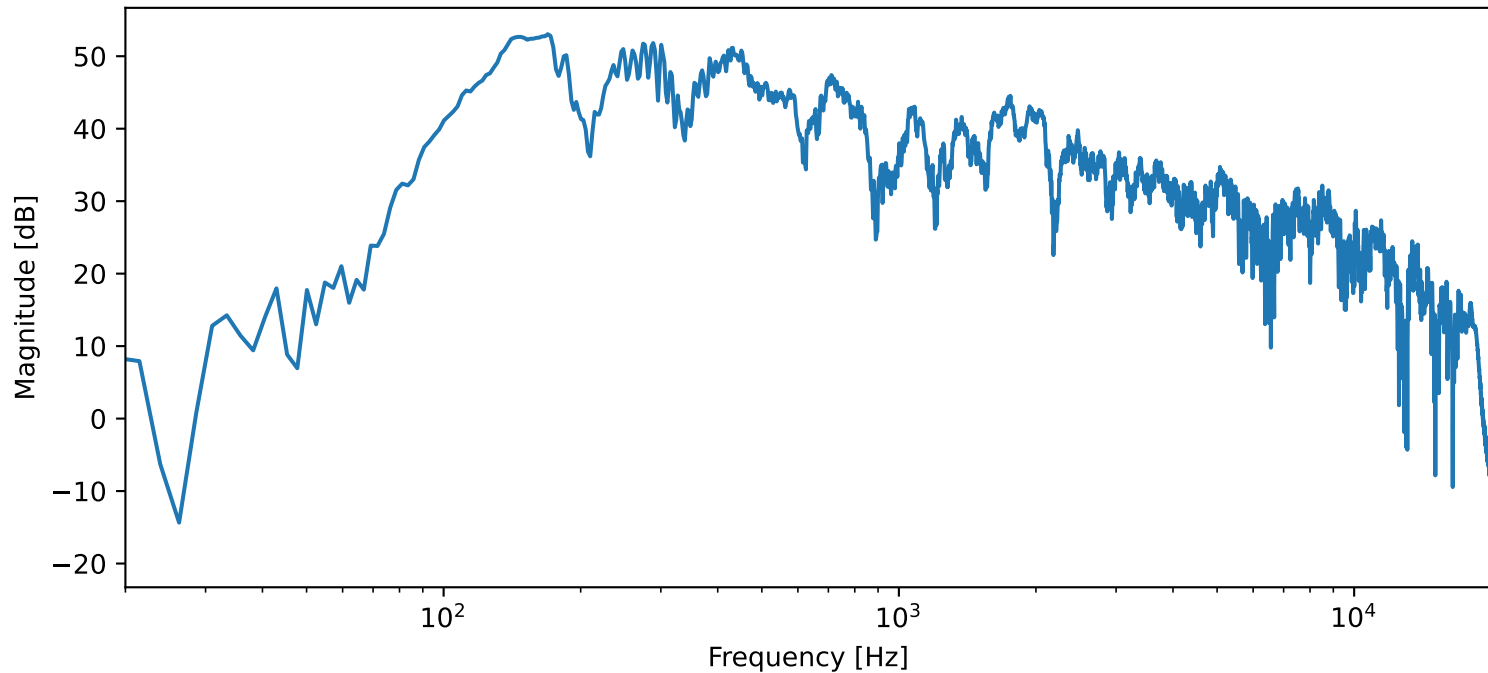
FFT of trimmed recording — 227_6.6_320NW (Lar dec)
