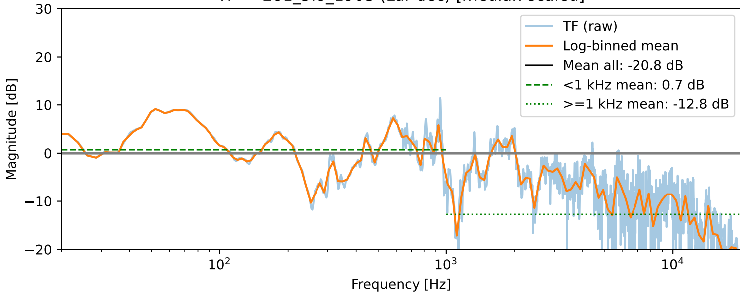
TF — 281_5.8_190S (Lar dec) [median-scaled]
