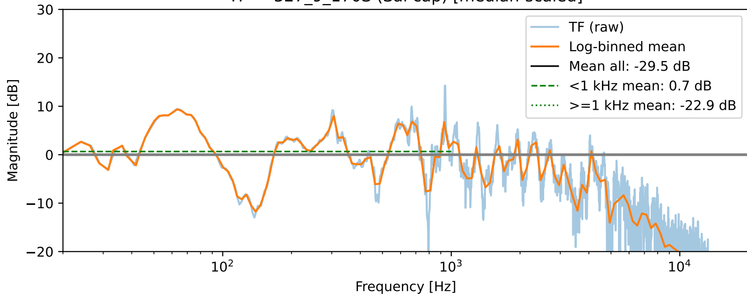
TF — 327_9_170S (Sal cap) [median-scaled]
