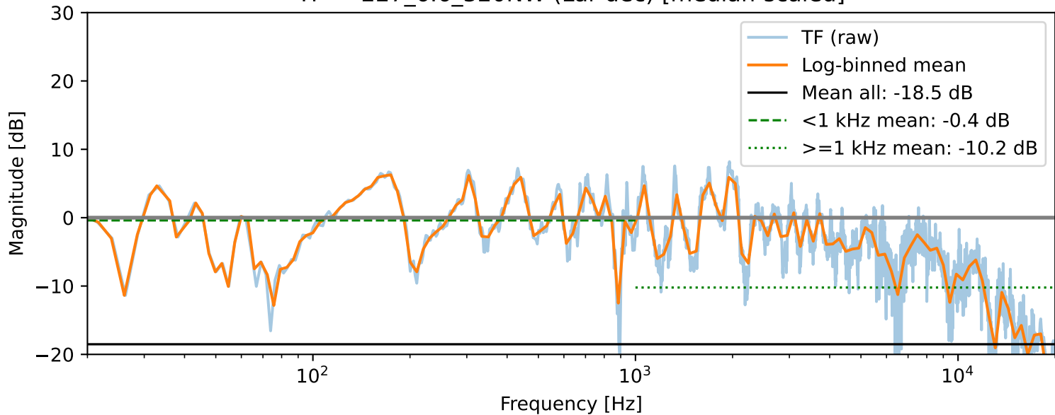
TF — 227_6.6_320NW (Lar dec) [median-scaled]
