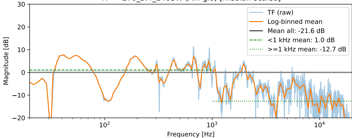
TF — 270_5.4_240SW (Aln glu) [median-scaled]
