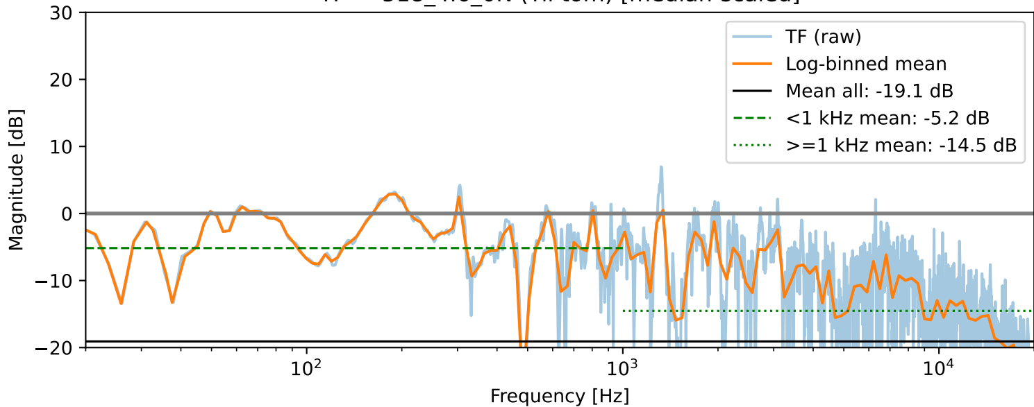
TF — 518_4.6_0N (Til tom) [median-scaled]
