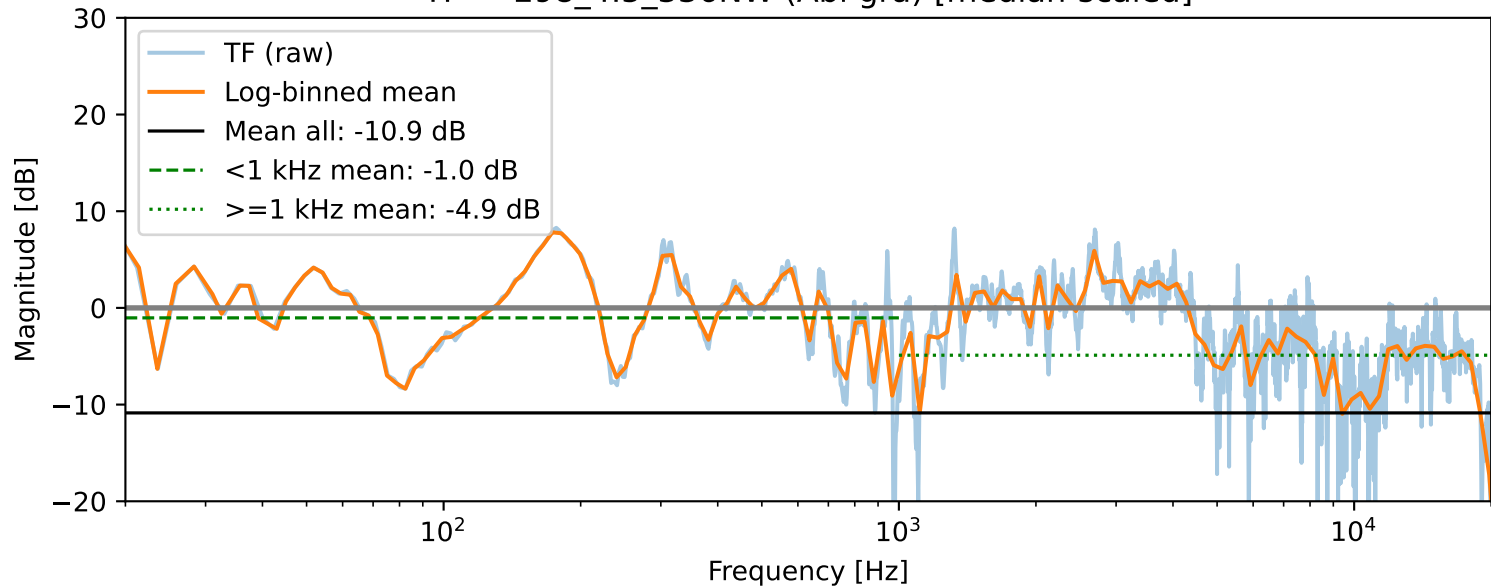
TF — 298_4.5_336NW (Abi gra) [median-scaled]
