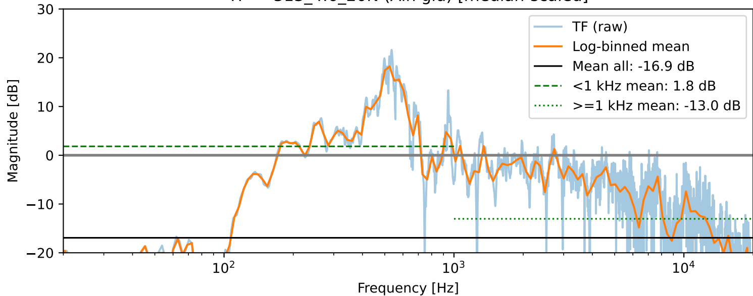
TF — 313_4.6_20N (Aln glu) [median-scaled]
