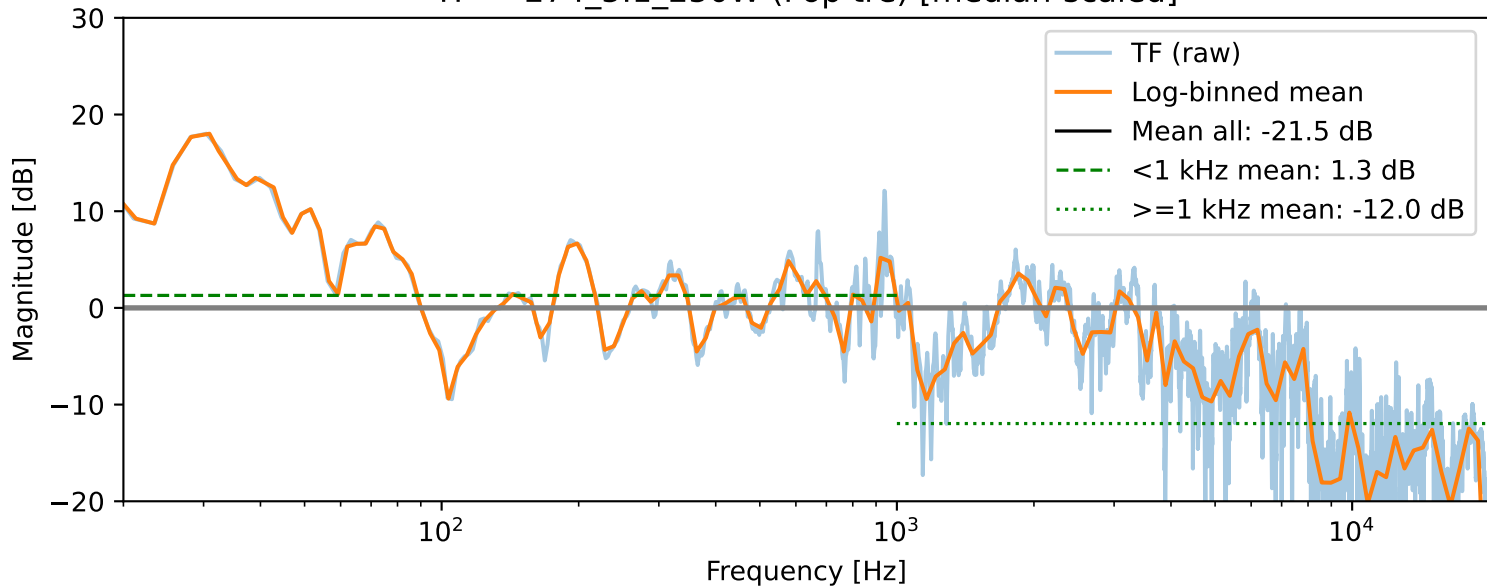
TF — 274_5.1_250W (Pop tre) [median-scaled]
