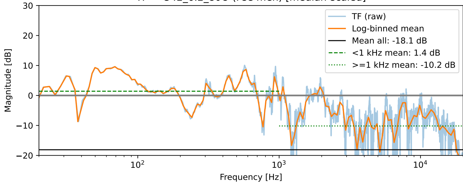
TF — 342_6.2_800 (Pse men) [median-scaled]
