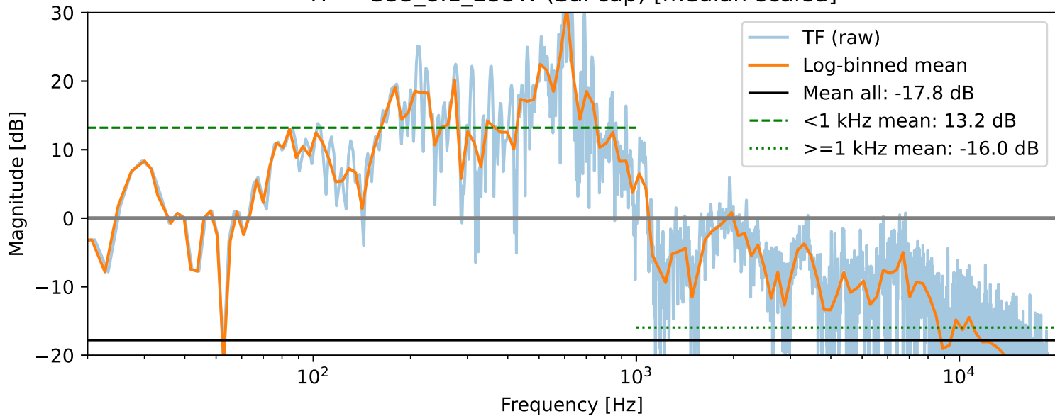
TF — 353_8.1_255W (Sal cap) [median-scaled]
