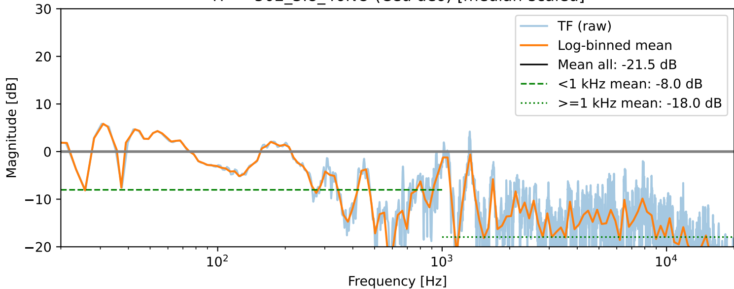
TF — 502_3.8_46NO (Ced deo) [median-scaled]
