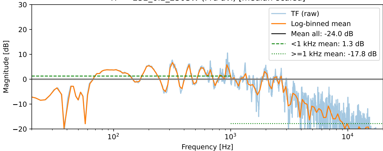
TF — 232_6.2_230SW (Pru avi) [median-scaled]
