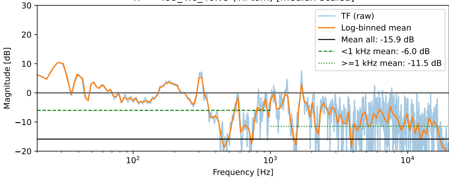
TF — 499_4.6_40NO (Til tom) [median-scaled]
