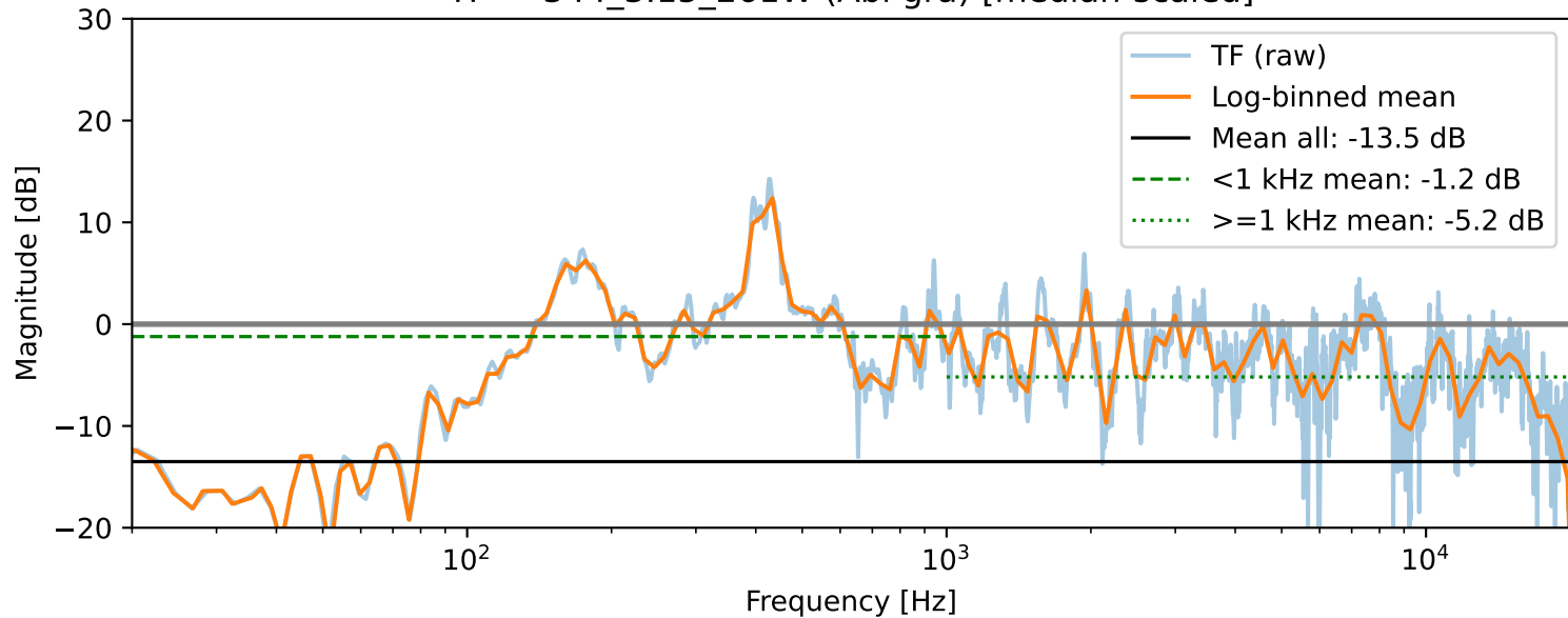
TF — 344_3.15_261W (Abi gra) [median-scaled]
