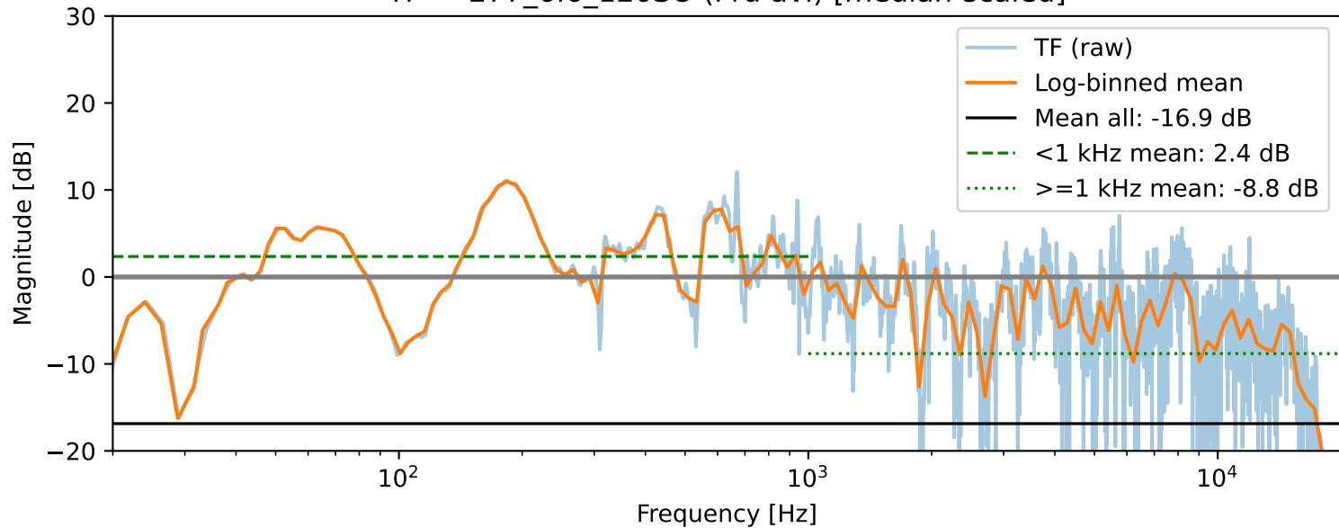
TF — 277_6.6_120SO (Pru avi) [median-scaled]
