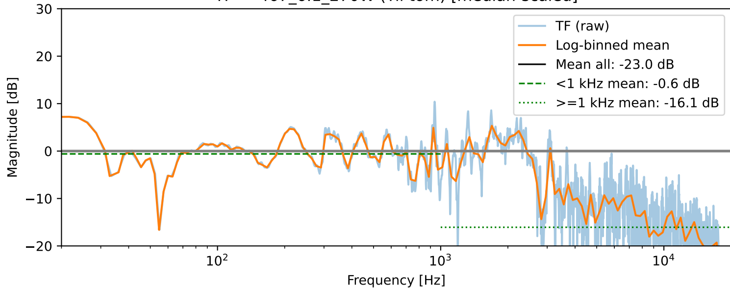
TF — 467_6.1_270W (Til tom) [median-scaled]
