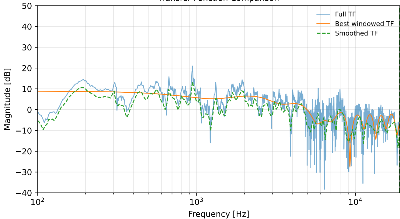
Transfer Function Comparison
