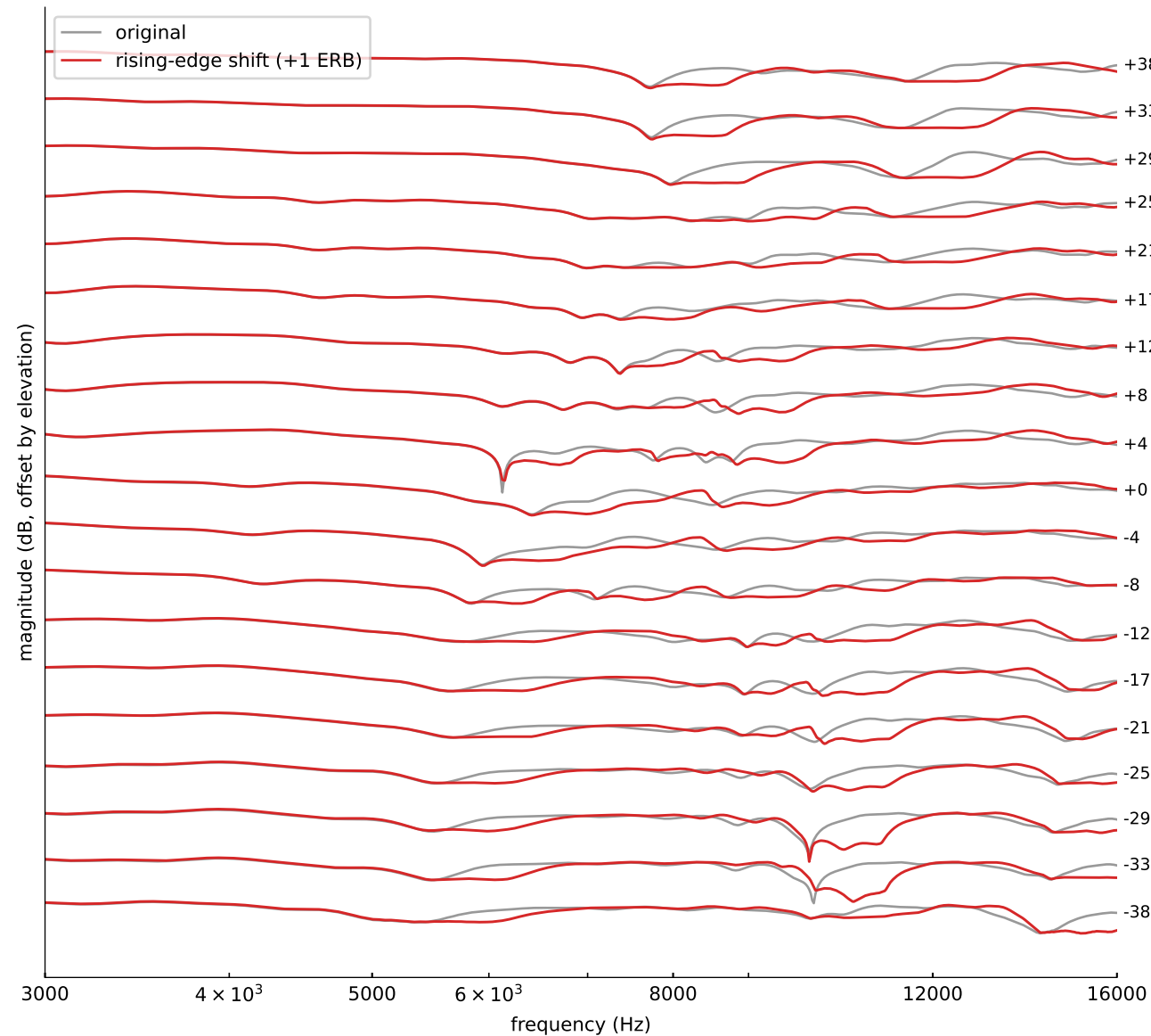
median-plane DTF (left ear) original vs rising-edge shift (+1 ERB)
