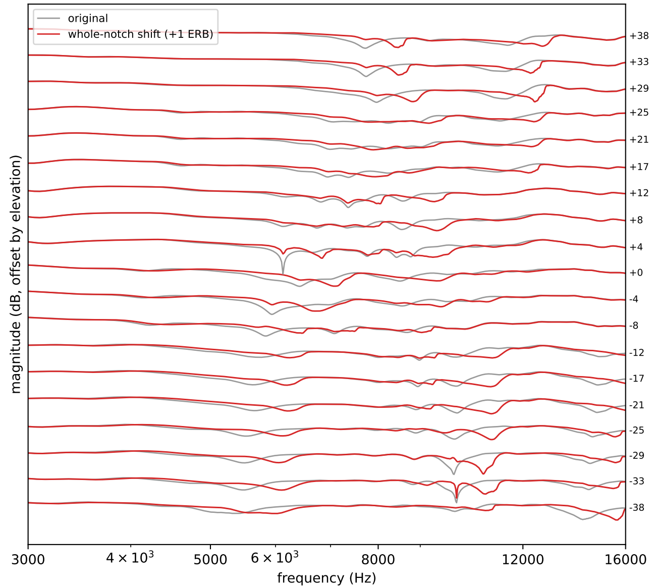
median-plane DTF (left ear) original vs whole-notch shift (+1 ERB)
