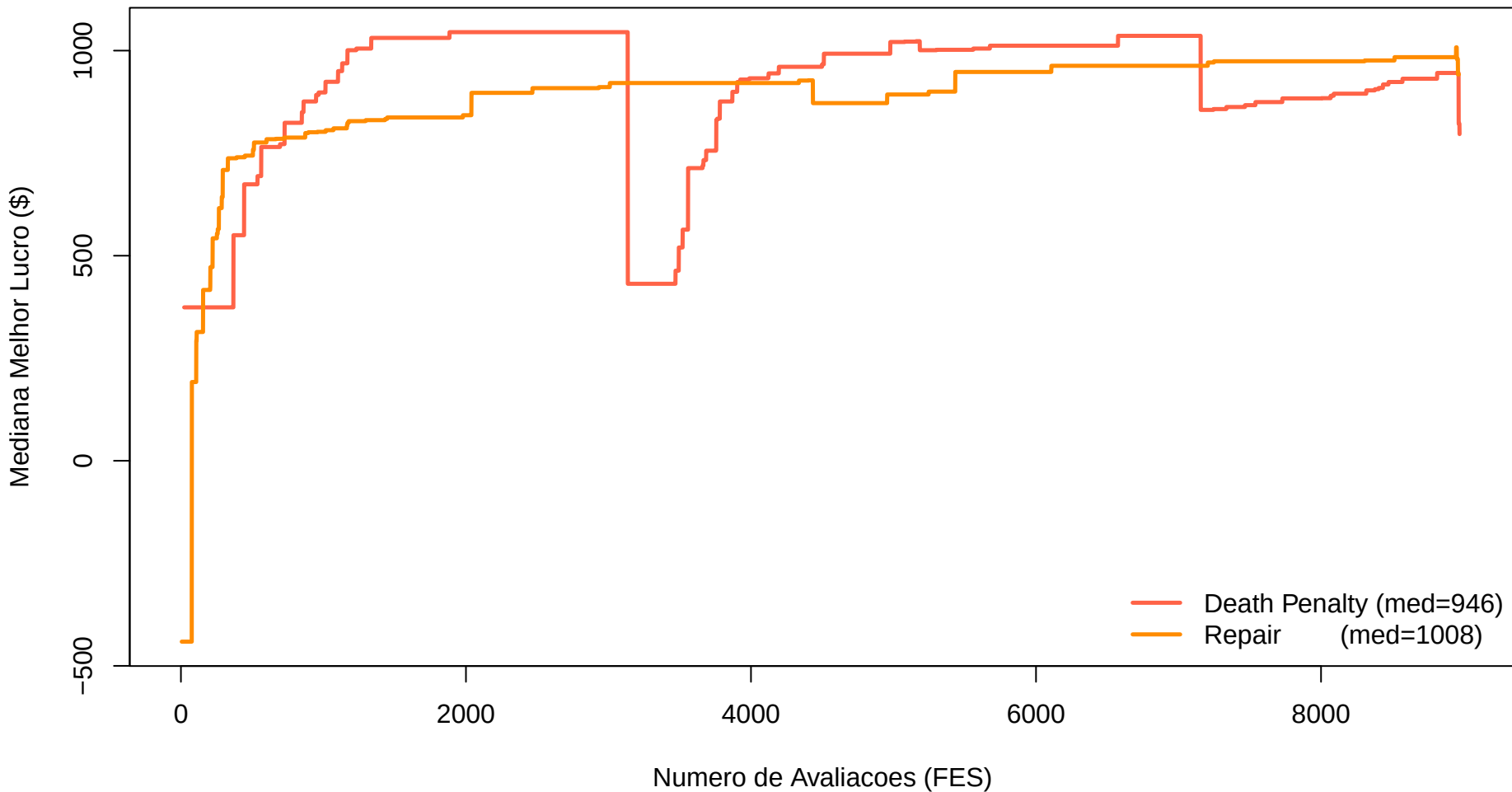
rbga.bin O2 – Death Penalty vs Repair (5 runs)
