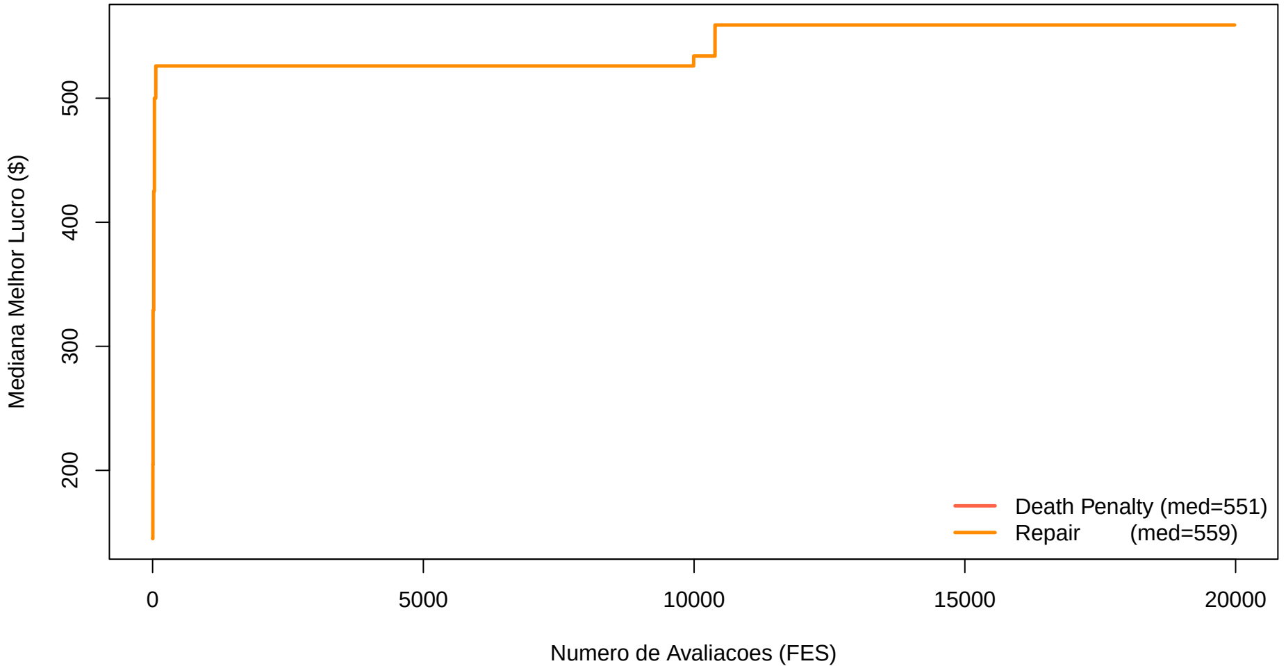
Tabu Search O2 – Death Penalty vs Repair (5 runs)
