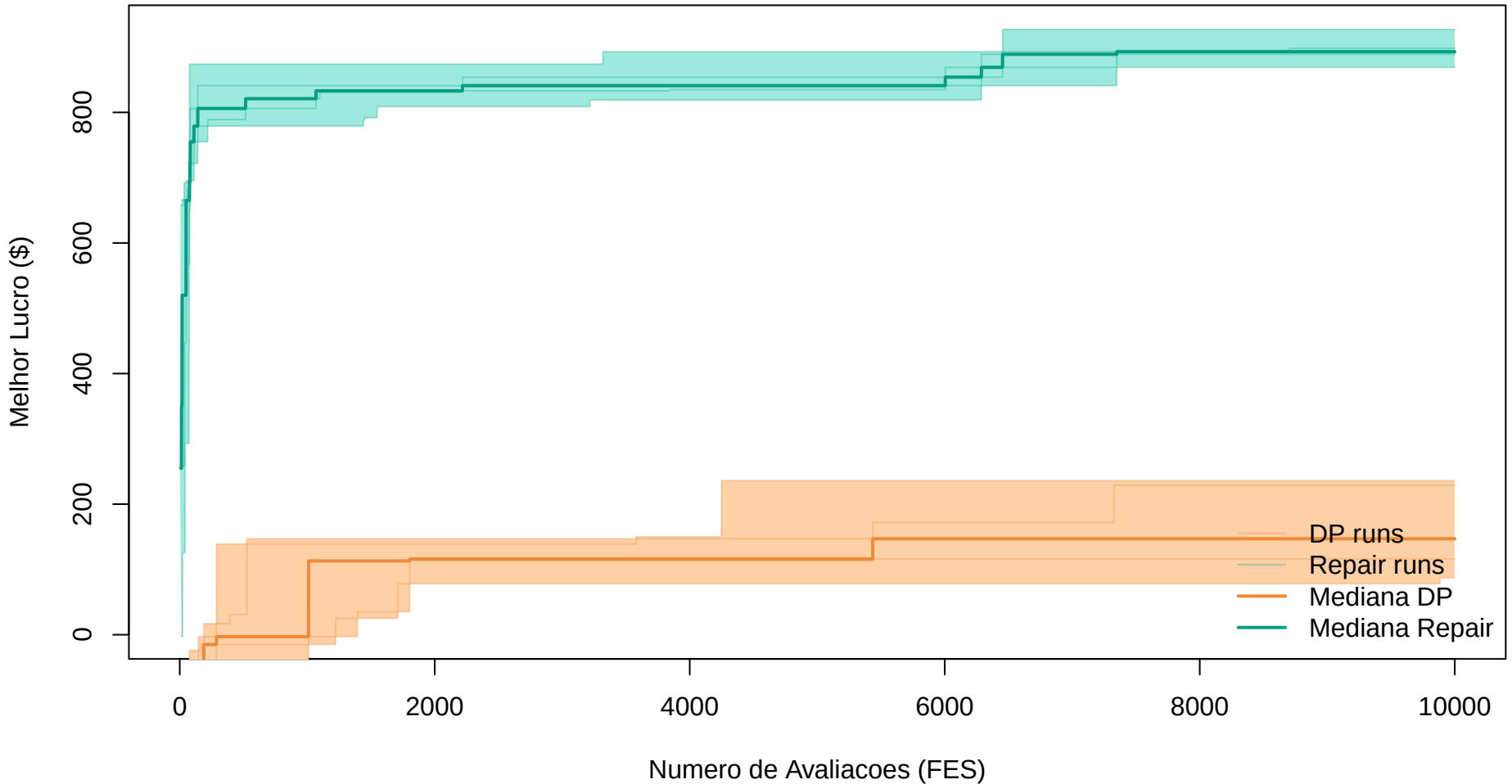
Monte Carlo O2 – Death Penalty vs Repair (5 runs)
