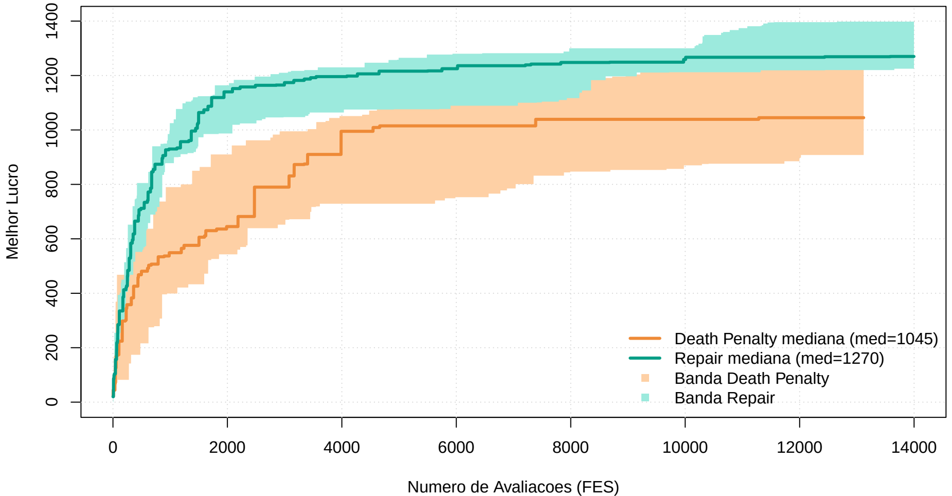
PSO O2: Death Penalty vs Repair – 5 runs
