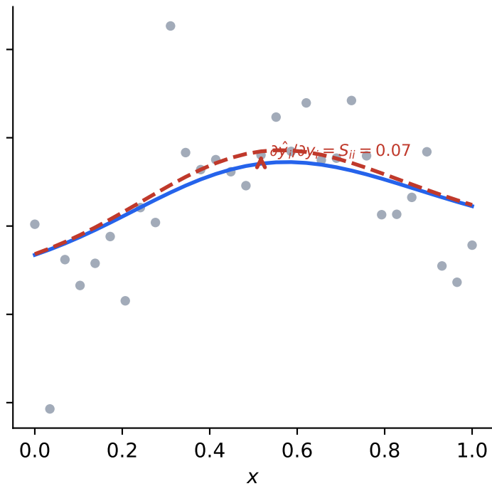
large bandwidth (smooths): S_{ij} \approx 0
