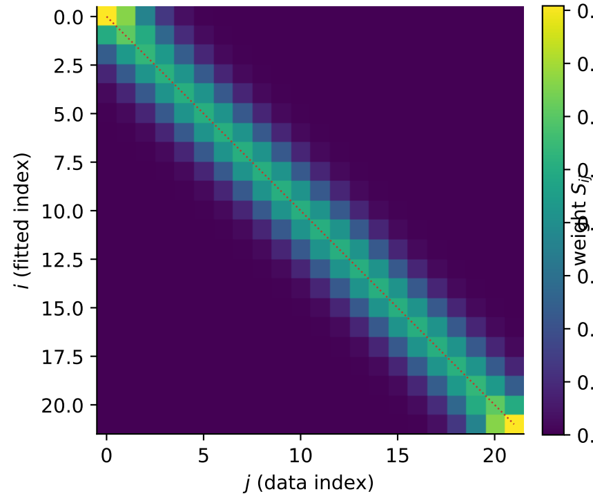
smoother matrix S ( \hat{y} = Sy ); df = \text{tr } S = 6.01
