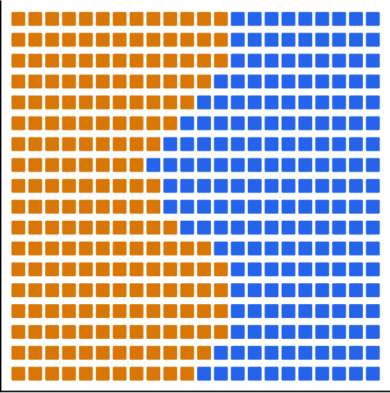
true field
