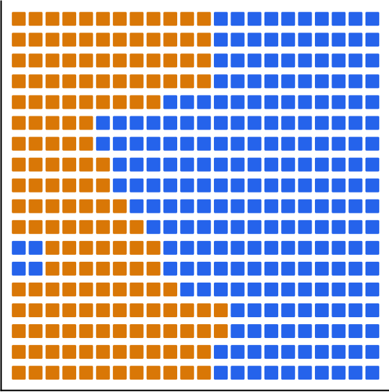
graph-regularized field
