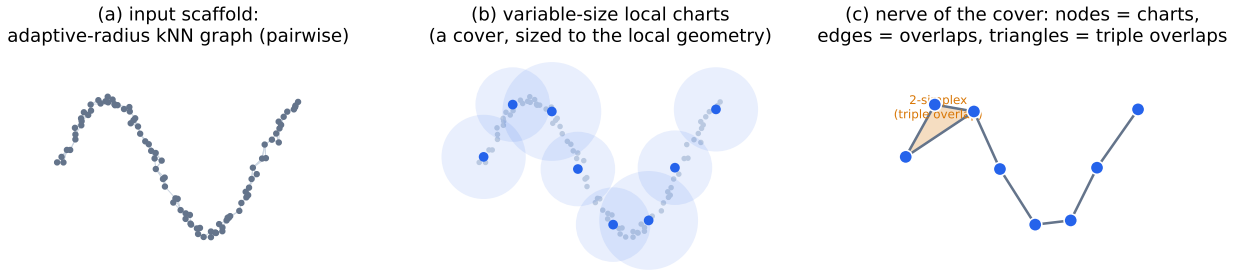
Figure 1: The shift in substrate. (a) The input scaffold: an adaptive-radius kNN graph, pairwise and fixed before estimation. (b) The charts form a cover whose pieces can vary in size with the local geometry. (c) The nerve of that cover: charts are nodes, an edge marks a pairwise overlap, and a filled triangle marks a place where three charts overlap at once — structure a pairwise graph cannot record.
