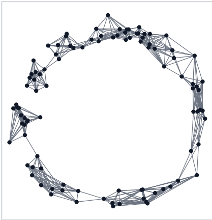
PHATE
