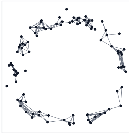
mKNN
