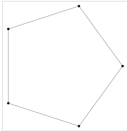
mKNN
