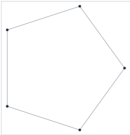
PHATE
