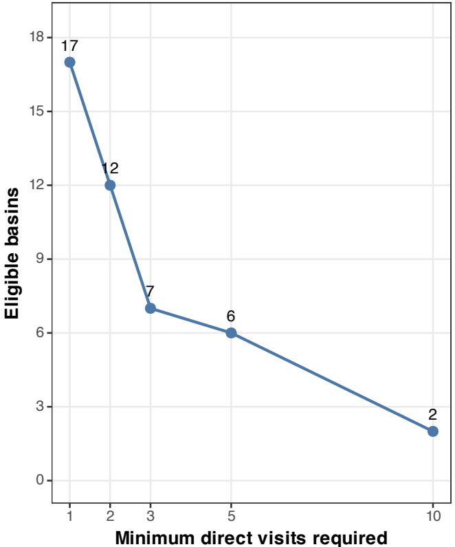
A. Number of retained candidate basins
