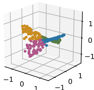
Stress MDS
