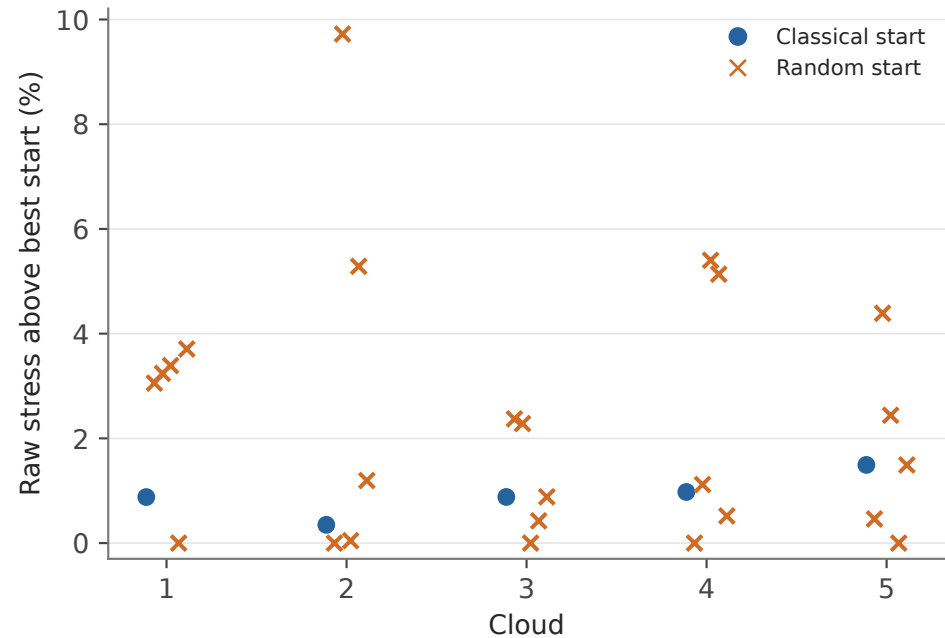
Six starts at each selected graph
