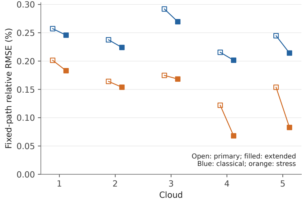
Additional 1,000 uniform edge-KK steps
