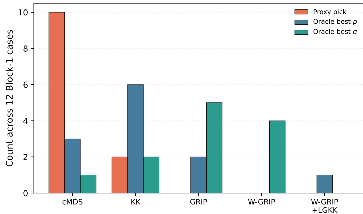
Phase E Block 1 seed-selection mismatch
