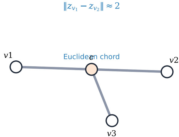
(b) Euclidean-output fit
