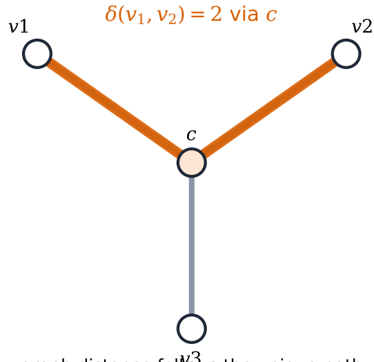
(a) Input graph metric
