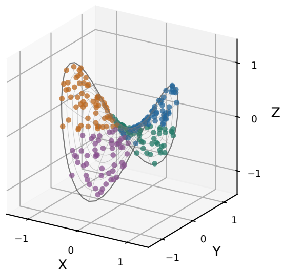
Original surface r = 64
