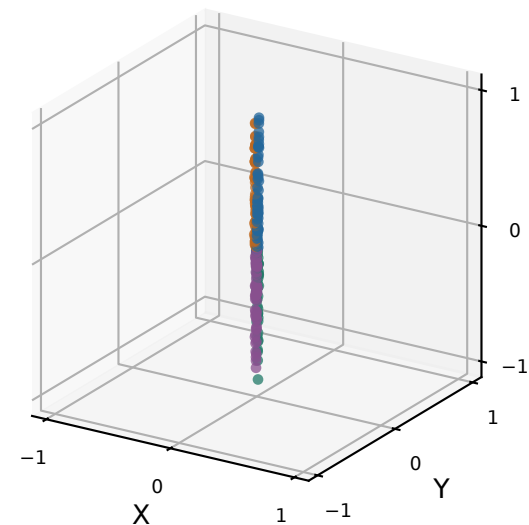
Ambient graph + edge-KK r = 64
