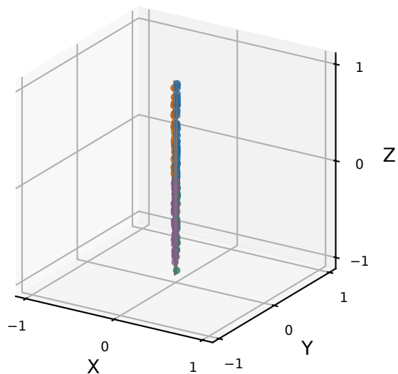
Original surface r = 64
