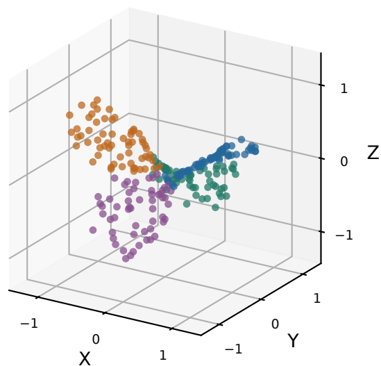
Geodesic graph + edge-KK r = 64
