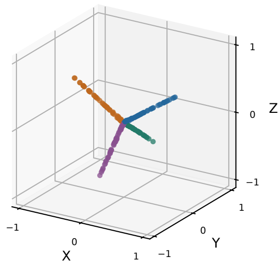
Geodesic graph + edge-KK r = 64
