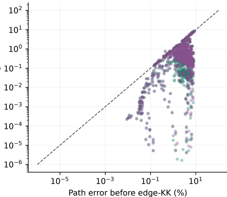
Path error after edge-KK (%)
