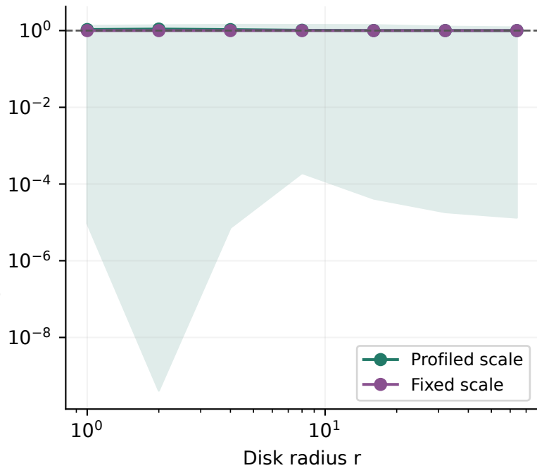
Edge calibration factor b
