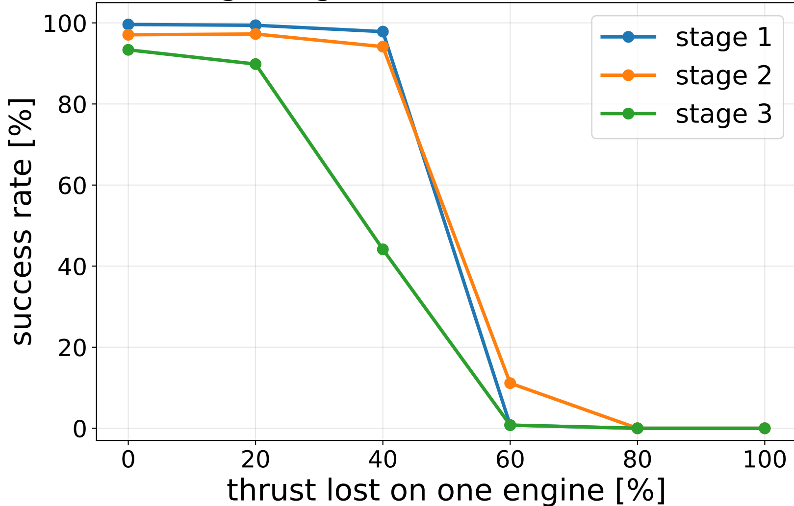
Single-engine thrust loss (zero-shot)
