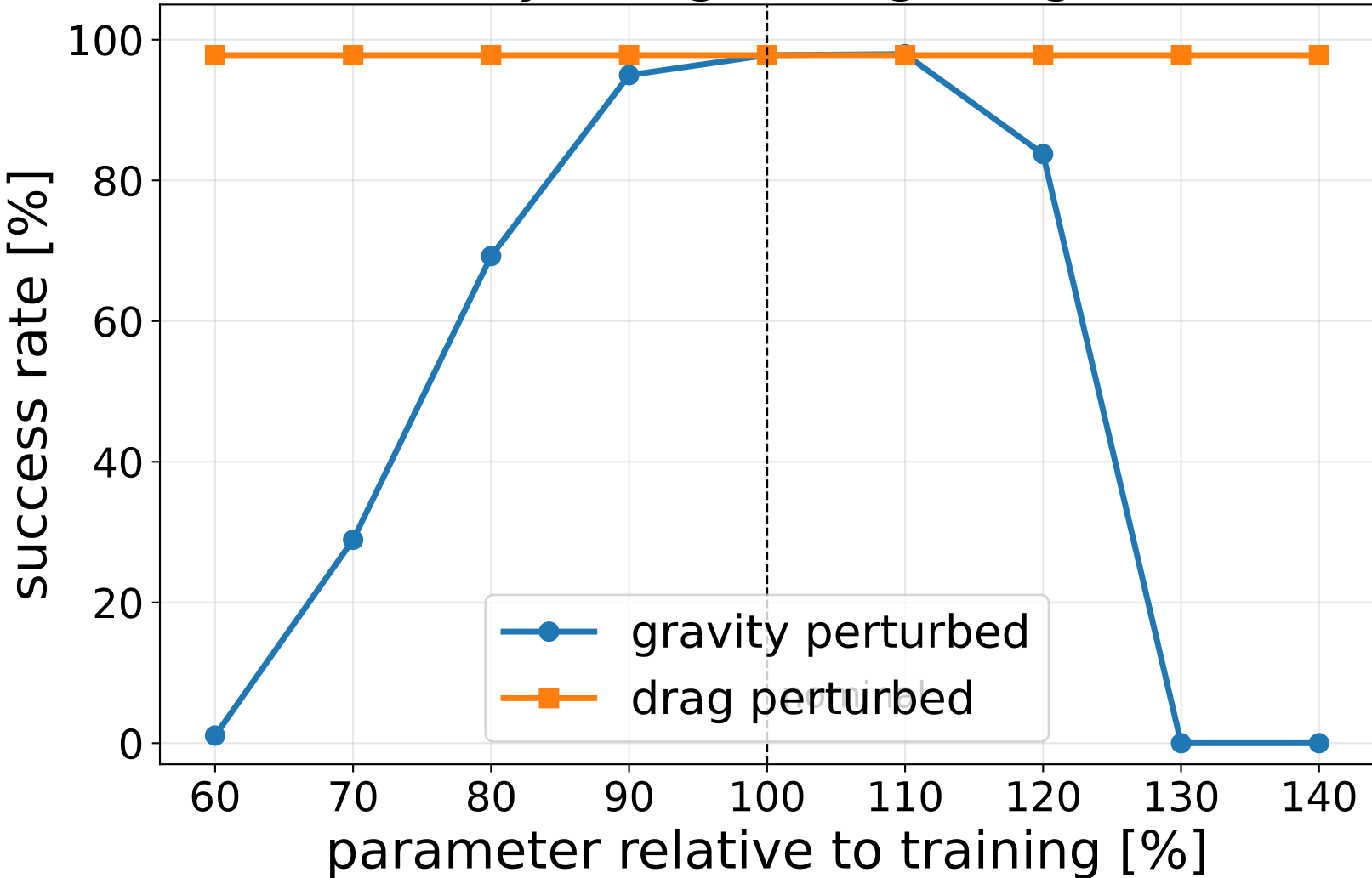
Gravity / drag scaling (Stage 2)
