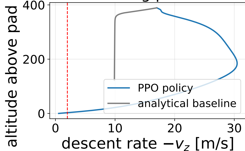
Braking profile
