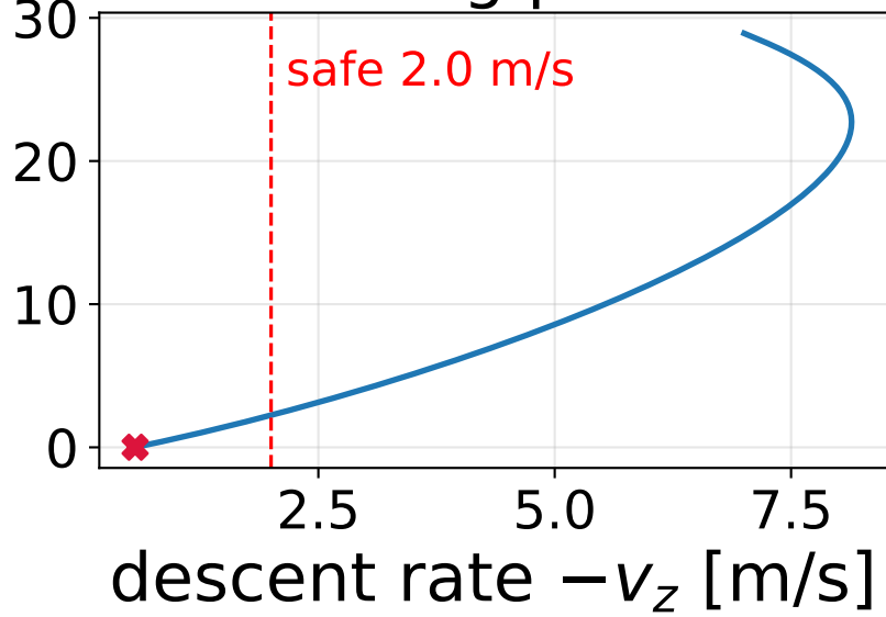
Braking profile
