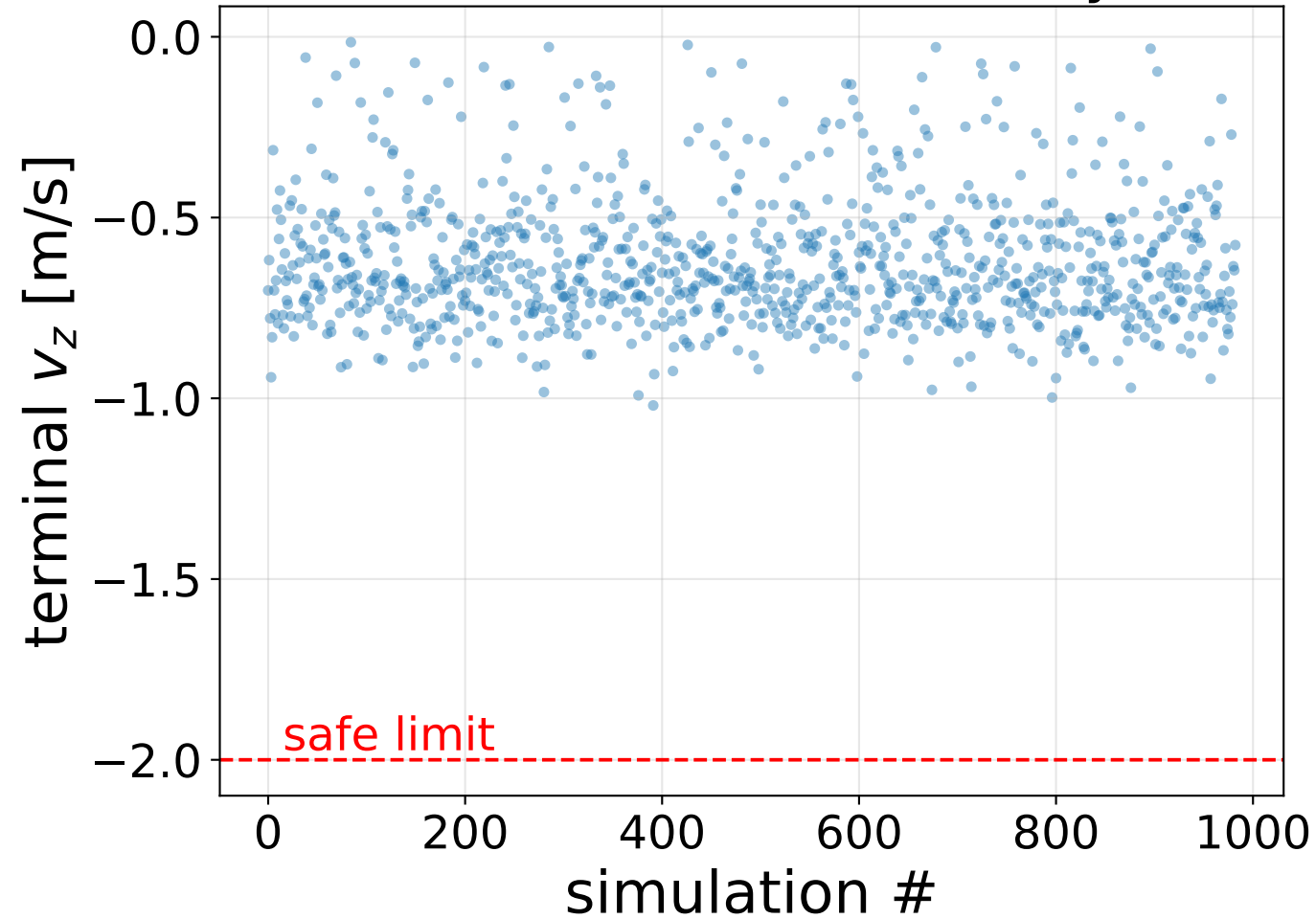
Terminal vertical velocity
