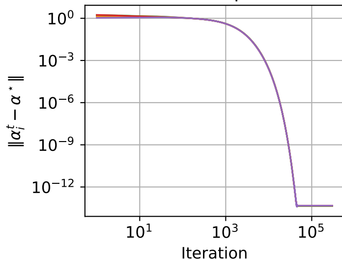
Dual decomposition
