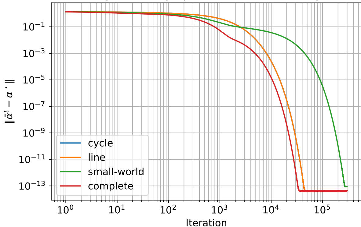
Dual decomposition - graph effect on the averaged iterat
