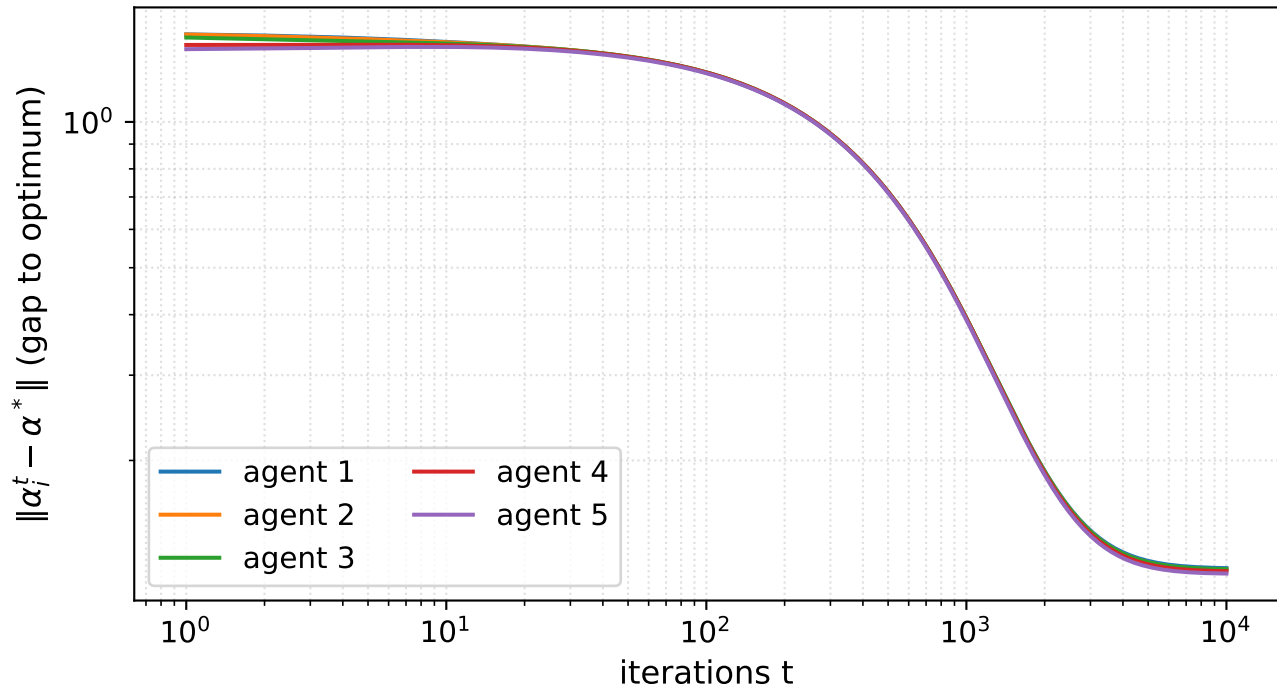
Decentralized gradient descent (line), eta=1.83e-03
