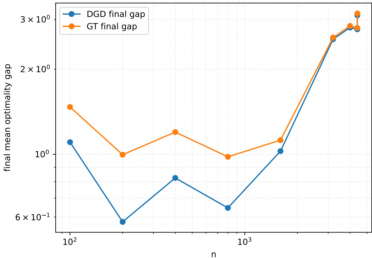
Probe convergence quality vs n
