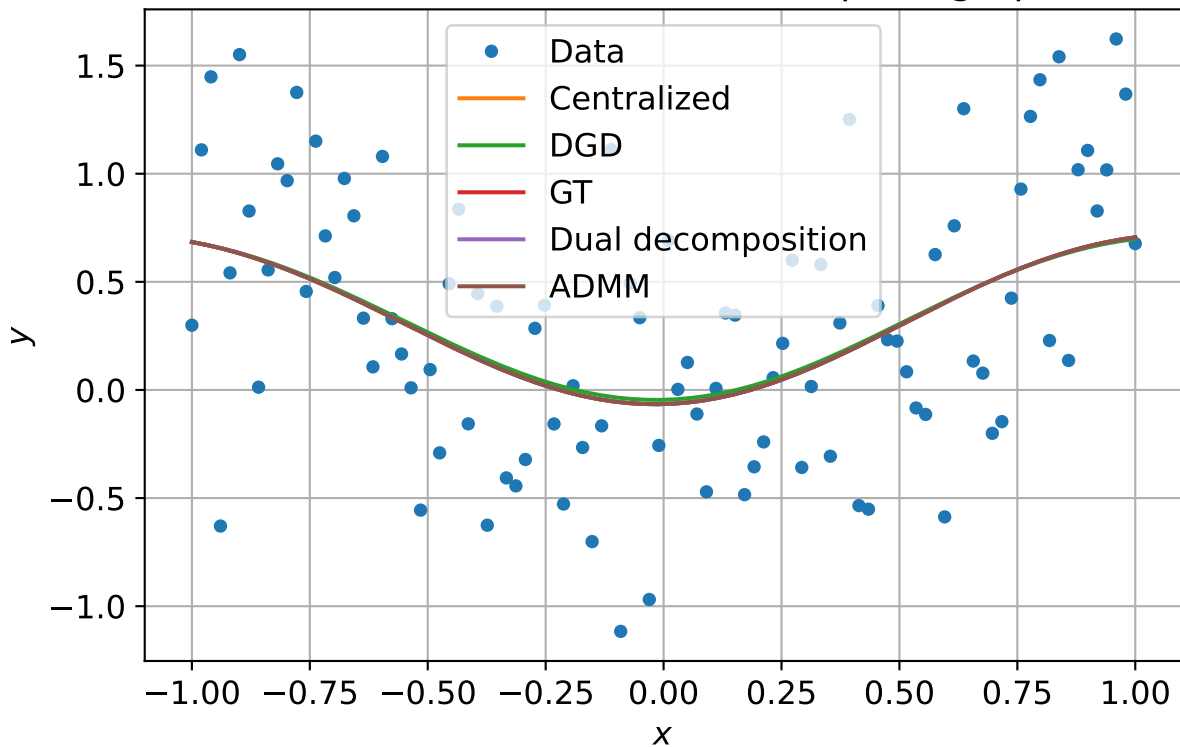
Function reconstruction - complete graph
