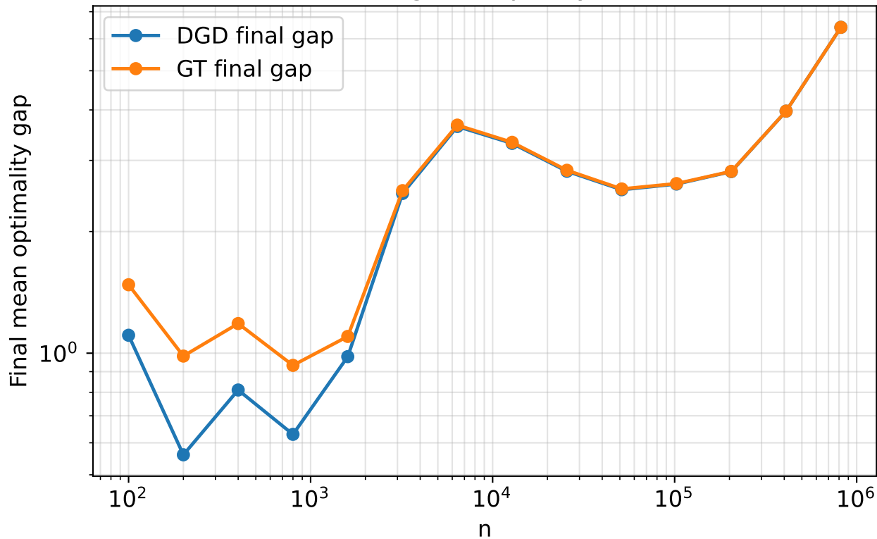
Convergence quality vs n
