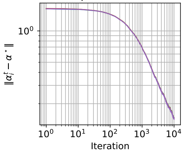
epsilon=10.0
