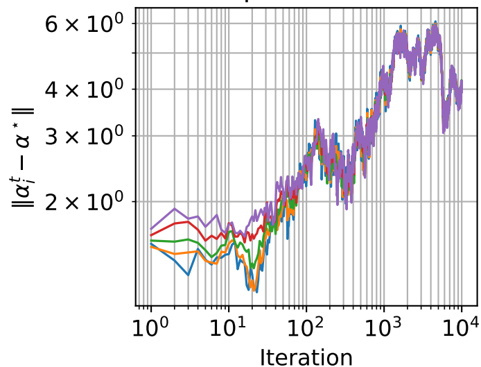
epsilon=0.1
