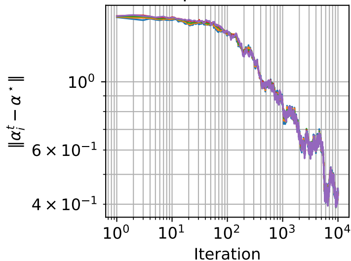
epsilon=1.0
