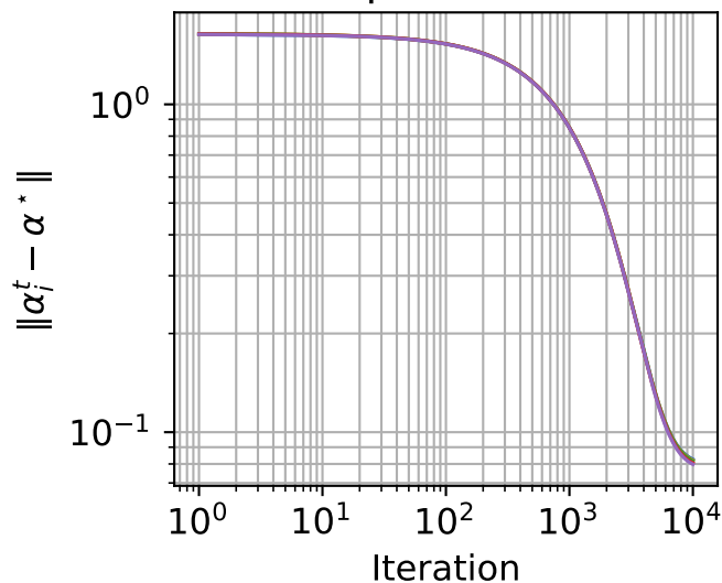
Non-private DGD
