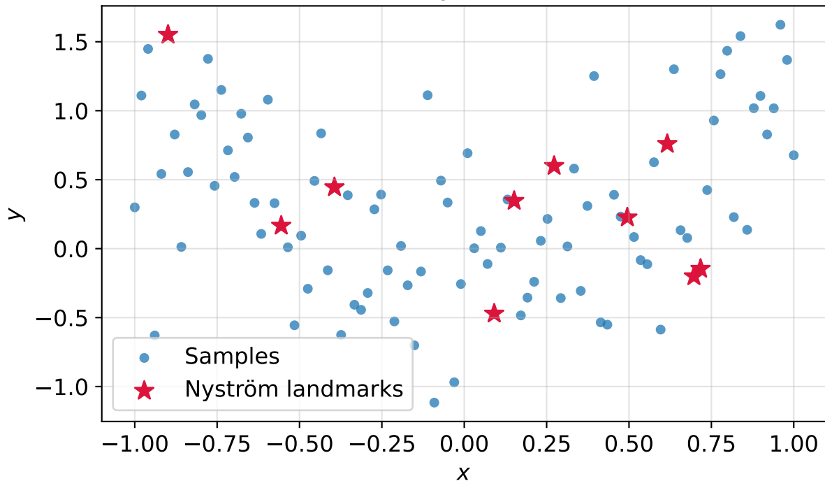
Dataset and Nyström landmarks
