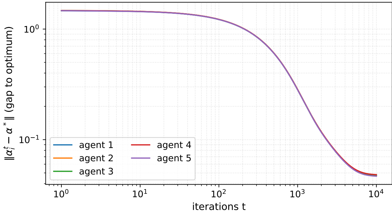
Decentralized gradient descent (fully-connected), eta=1.83e-03
