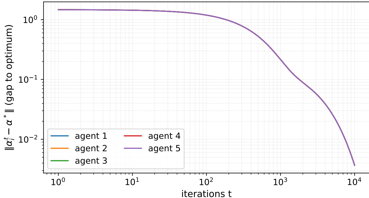
Gradient tracking (fully-connected), eta=1.83e-03
