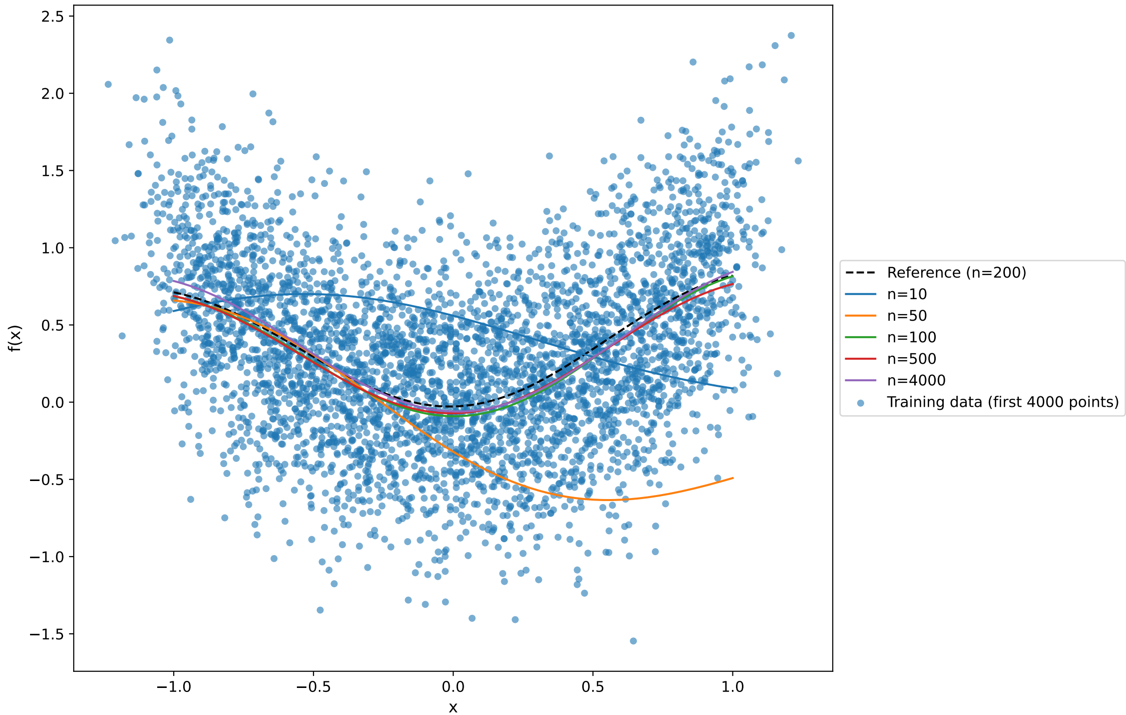
Reconstructed functions for different n (fixed landmarks)
