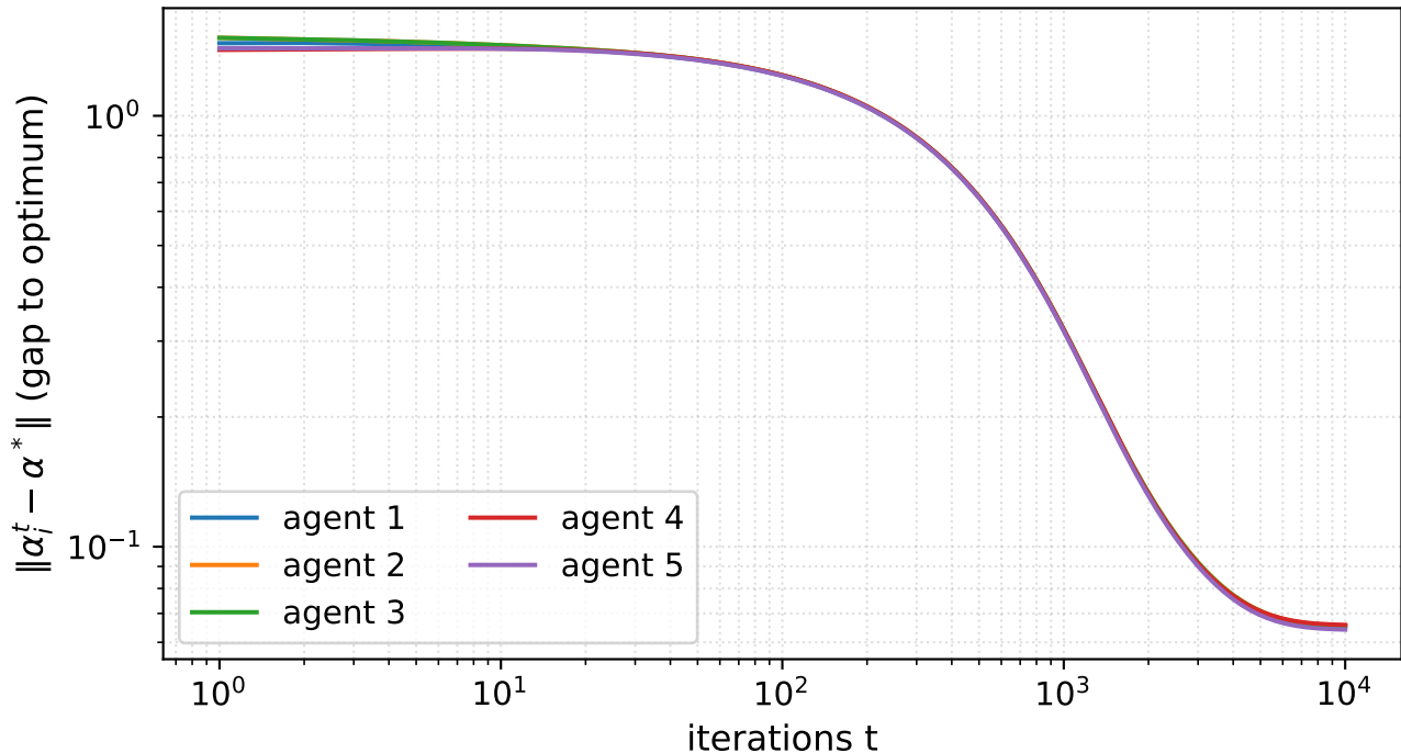
Decentralized gradient descent (small-world), eta=1.83e-03
