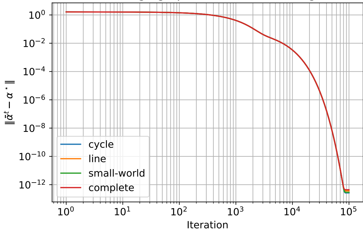
Gradient tracking - graph effect on the averaged iterate
