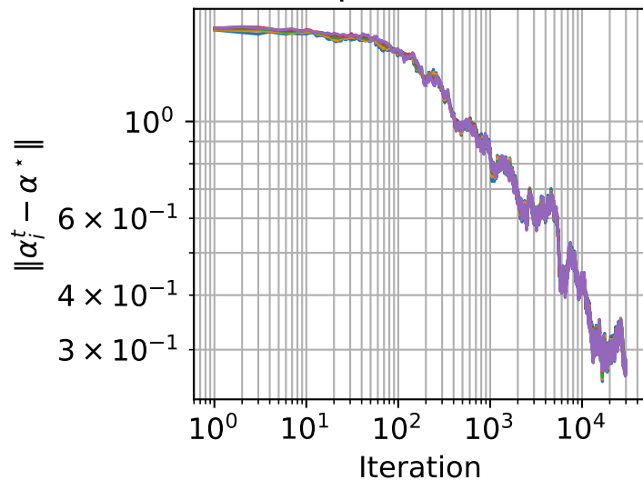
epsilon=1.0
