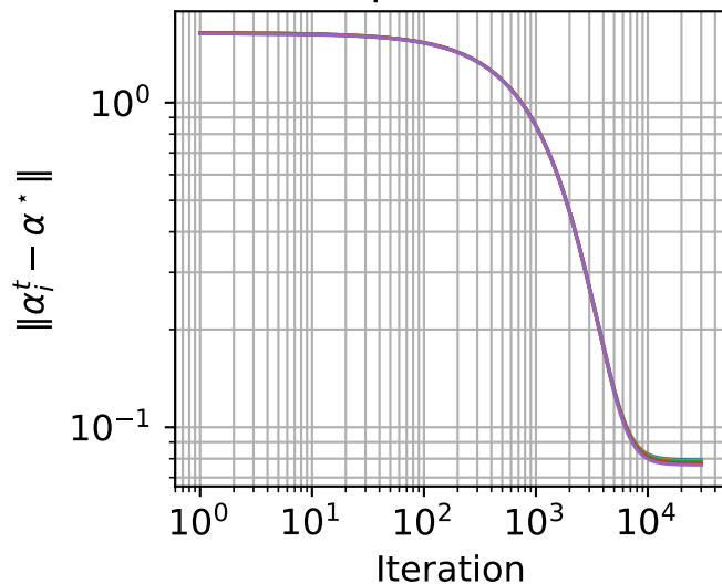
Non-private DGD
