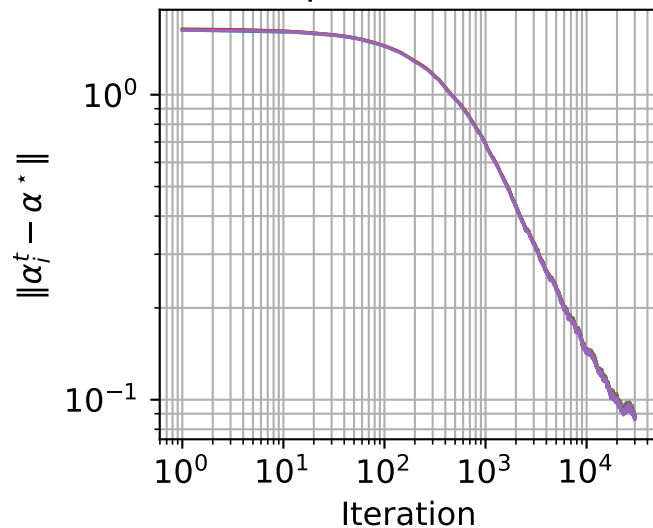
epsilon=10.0
