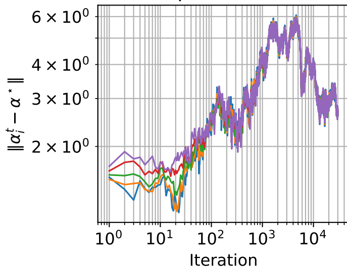
epsilon=0.1
