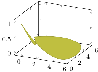
Faceted + 0 refines
