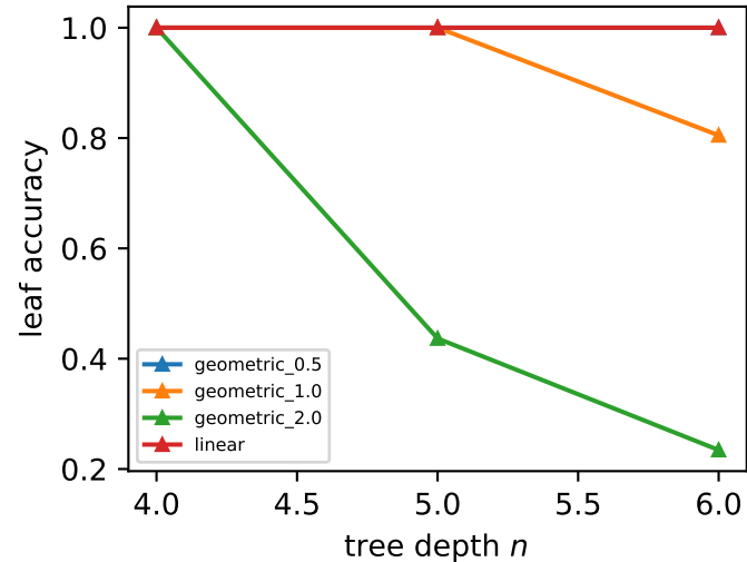
(c) profile choice vs accuracy, p = 3
