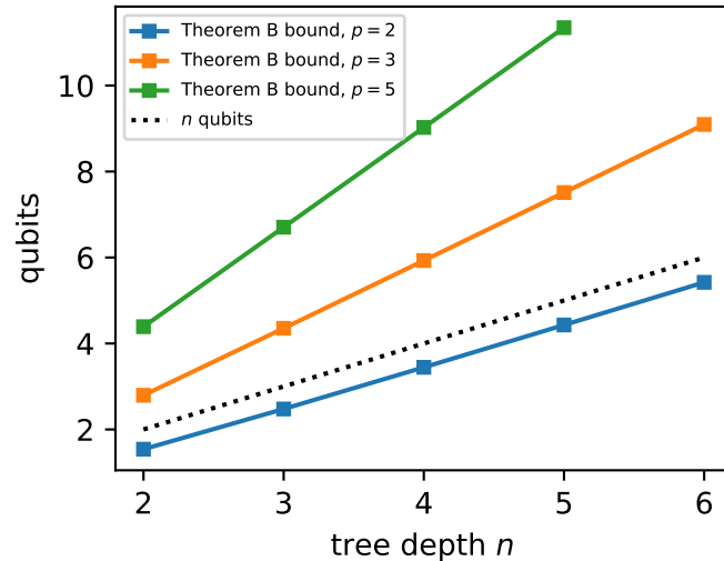
(b) Theorem B crossing (full tree)
