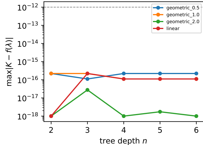
(a) exactness is not fragile
