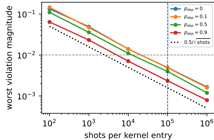
(a) sampling variance, and it decays
