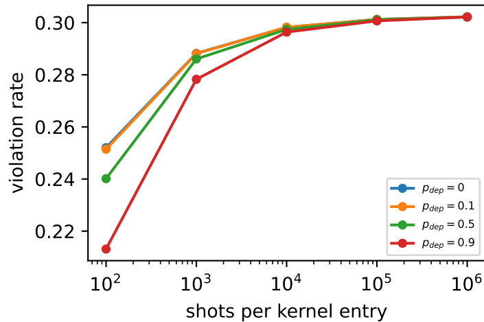
(b) but the count saturates: ties
