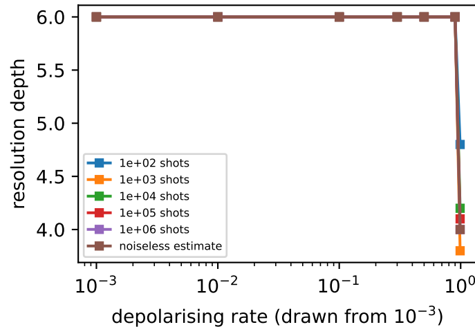
(c) depolarising bias flattens the profile
